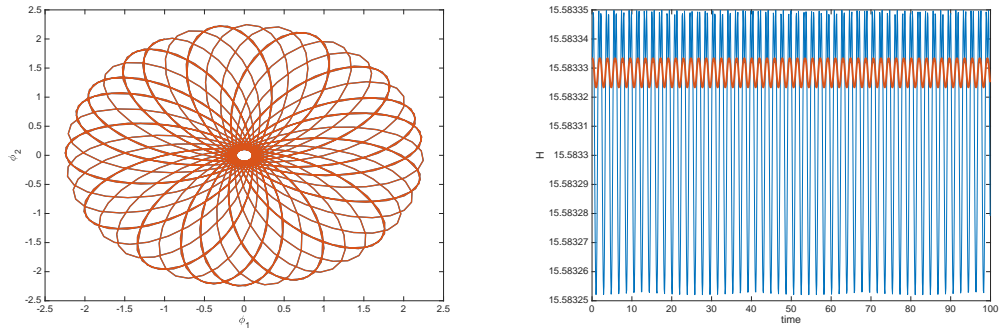
(a) Phaseplot motion in modified system (b) H along motion in exact/modified system
