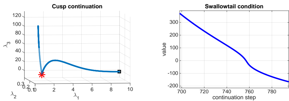
Figure 11.4: The left figure shows a continuation of the cusp singularity detected in Figure 11.1 by varying \lambda_1 , \lambda_2 and \lambda_3 . A swallowtail point is marked by * . The square marker shows where the continuation was initiated. As the line of cusps is numerically continued the swallowtail condition is monitored. To the right we see the value of the swallowtail condition versus the number of continuation steps. The root corresponds to the swallowtail point. Since the root is nondegenerate, we know that the butterfly condition is not fulfilled such that the singularity is indeed a swallowtail point and not further degenerate.
