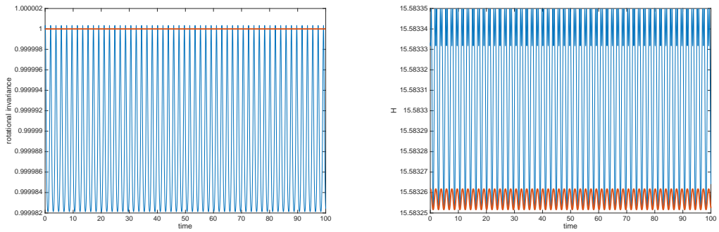
(c) I_{\text{rot}} along motion in exact/modified system (d) H and H_{\text{corrected}} modified system
