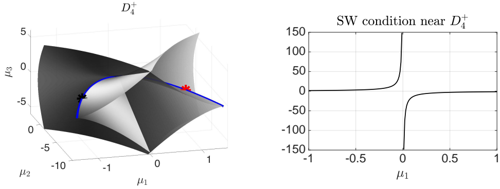
Figure 11.2: The left figure shows a singularity of type D_4^+ , called hyperbolic umbilic singularity . It is a generic codimension 3 singularity in catastrophe theory. Here \mu = (\mu_1, \mu_2, \mu_3) are parameters. Each point on the blue line (the edge) corresponds to a cusp singularity with an exception at \mu = (0, 0, 0) where the D_4^+ singularity is located. The two points marked with asterisks are cusp points with different signatures. The figure to the right shows the value of the bifurcation test equation for A_4 along the line of cusps parametrised by \mu_1 . We see that the bifurcation test equation has a singularity at \mu_1 = 0 , where the hyperbolic umbilic singularity is located, and that it changes sign at the singularity.
