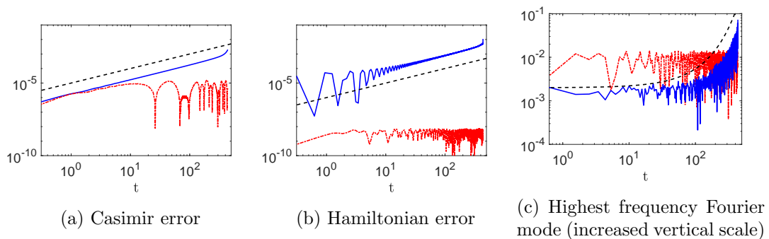
Figure 12.6: The errors corresponding to the conventional (—) and collective (---) methods for the travelling wave experiment. The reference lines (---) are \mathcal{O}(t) in figures (a) and (b) and exponential in figure (c).
