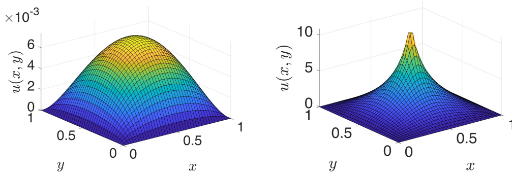
Figure 4.1: Plot of a high- and low energy solutions to the Bratu problem for the parameter value \mu = 0.1 using 6400 interior grid points.
