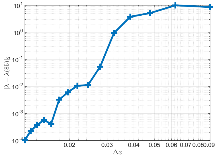
Figure 11.7: Euclidean distance of the parameter (\lambda_1, \lambda_2, \lambda_3) to the calculated value at N = 85 as a function of the inner grid spacing \Delta x = \frac{1}{N+1} . Here N is the number of inner grid points per dimension N with N = 10, 15, \dots, 80, 85 . In each step the position of \lambda is obtained by calculating a root of F^{(3)}(u, \alpha, \bar{v}, \lambda) using Newton iterations until convergence ( \infty -norm smaller 10^{-9} ). We see that the values converge as \Delta x decreases.
