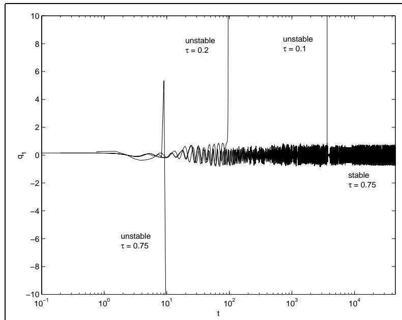
Figure 5: ABA leapfrog with 2 different initial conditions and different time steps. The ‘stable’ initial condition is q = 0, p = (\frac{1}{\sqrt{6}}, \frac{1}{\sqrt{6}}) , at the center of Fig. 3. The ‘unstable’ initial condition is q = (0.1, -0.5), p = 0 , on the base of the triangle in Fig. 3.
