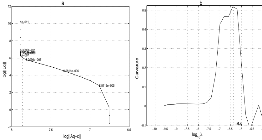
Figure 32: This figure demonstrates the use of maximum curvature method to estimate the optimal value of a regularisation parameter: (a) non-linear L-curve, (b) regularization parameter \lambda vs curvature
