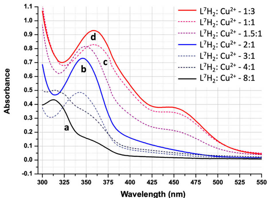
Figure 10. UV/Vis spectra of 80 \mu M solutions of L^7H_2 in MeCN containing varying concentrations of Cu(OAc)_2 \cdot H_2O ( L^7H_2 to Cu^{2+} molar ratio ranging from 1:3 to 8:1).
