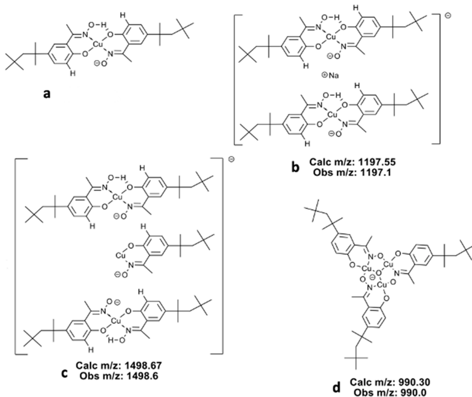
Figure 6. Suggested structures, together with their observed and calculated monoisotopic masses, for the dominant monoanionic species (a–d) in an acetonitrile solutions with different Cu(II):L^4H_2 molar ratios.
