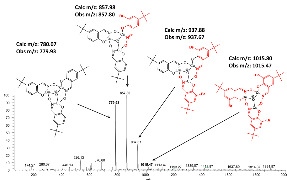
Figure 9. The mass spectrum obtained from a MeCN solution of Cu(II) acetate (50 \mu M) and L^6H_2 and L^8H_2 (each 25 \mu M). Proposed structures are inset with observed and calculated monoisotopic masses.
