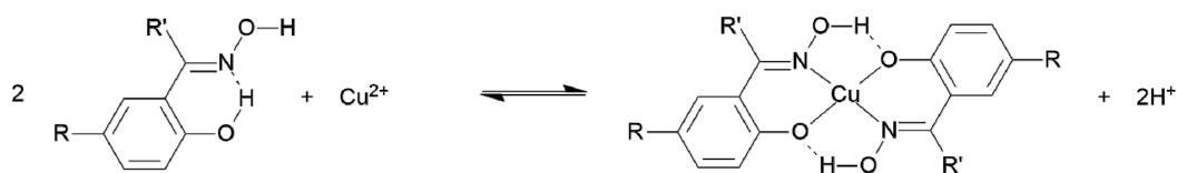
Figure 1. The pH-dependent extraction of Cu(II) by phenolic oximes.
