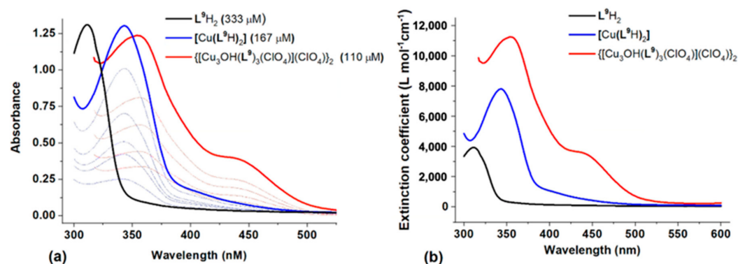
Figure 12. (a) The UV/Vis absorption spectra for varying concentrations of L^9H_2 , [Cu(L^9H)_2] and [Cu_3OH(L^9H)_3(ClO_4)](ClO_4)_2 and (b) their respective molar extinction coefficients, obtained by the absorbance vs. concentration plots from (a).
