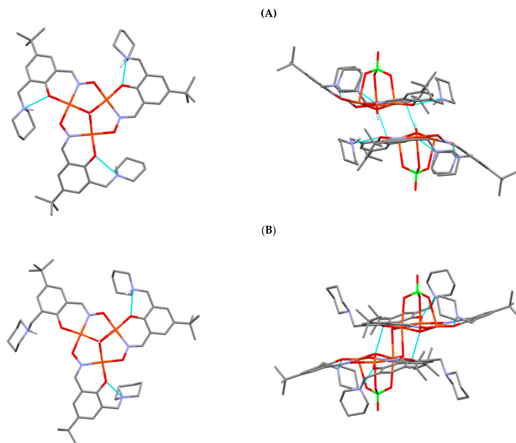
Figure 13. Components of the two crystalline forms ( A , B ) of the hexanuclear complexes \{[\text{Cu}_3\text{OH}(\text{L}^9\text{H})_3(\text{ClO}_4)](\text{ClO}_4)_2 \cdot 2\text{H}_2\text{O} \cdot 2\text{MeCN}\} and \{[\text{Cu}_3\text{OH}(\text{L}^9\text{H})_3(\text{ClO}_4)](\text{ClO}_4)_2 \cdot 11\text{H}_2\text{O} \cdot \text{MeCN}\} . The trinuclear entities [\text{Cu}_3\text{OH}(\text{L}^9\text{H})_3]^{2+} and the hexanuclear units [\text{Cu}_3\text{OH}(\text{L}^9\text{H})_3(\text{ClO}_4)]_2^{2+} are shown on the left and right, respectively. H-atoms not involved in H-bonding have been removed for clarity.
