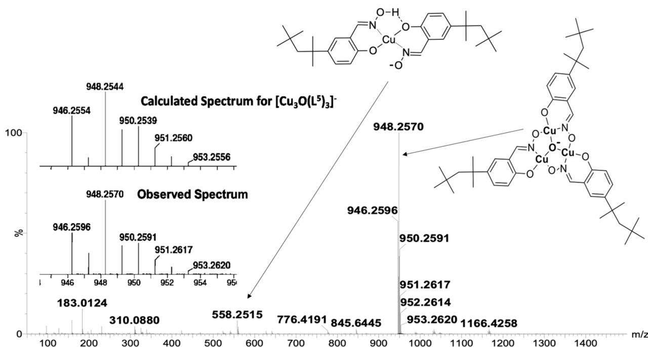
Figure 7. The high-resolution mass spectrum of a 50 \mu M solution of L^5H_2 and copper acetate in acetonitrile. The observed and the calculated isotopic peak distribution and masses for [Cu_3O(L^5)_3]^- are inset.
