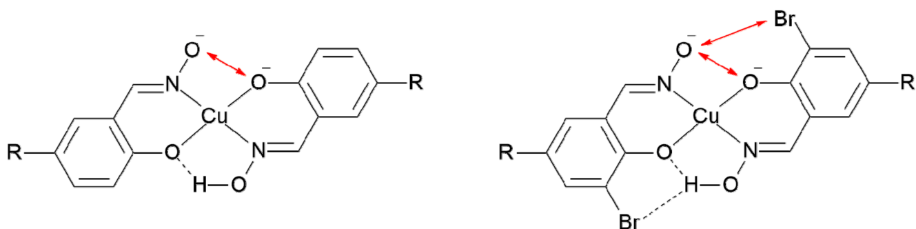
Figure 8. A representation of the origins of the stabilization of the monoanions [Cu(L)(LH)]^- by H-bonding in the lower part of the complexes (—) and of the destabilization by repulsion between electronegative atoms (double-headed red arrows in the upper part of the complexes).
