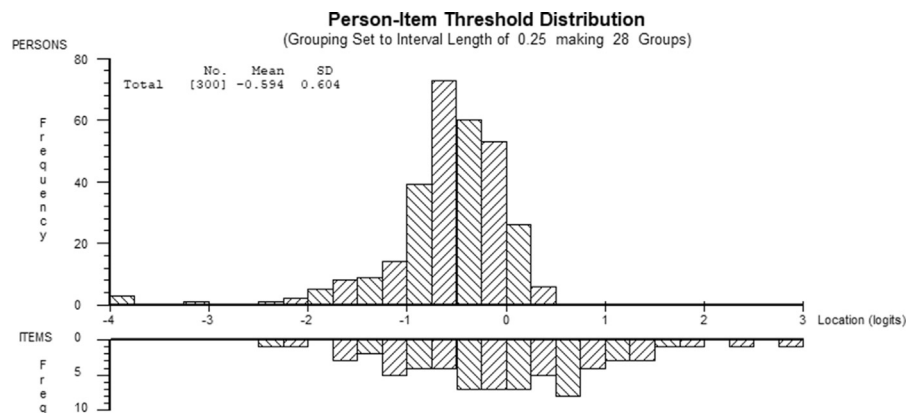
Fig. 1. Person-item threshold distribution.
