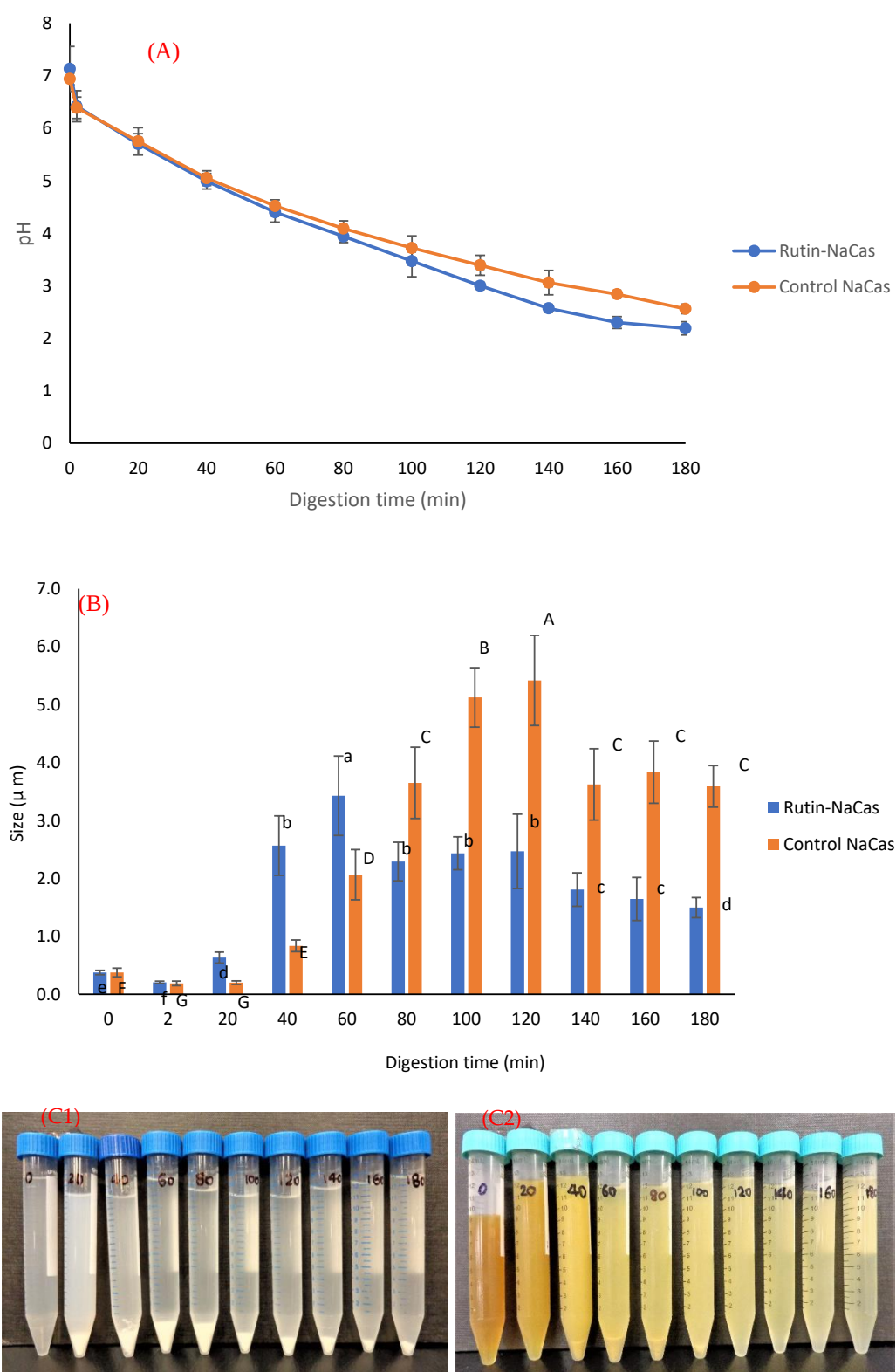
Figure 5. The behaviour of control NaCas and rutin–NaCas nanocomplexes (NaCas:rutin ratio of 2.5 w/w ) throughout the simulated gastric digestion. (A) pH profile; (B) particle size; (C) appearance (C1: control NaCas, C2: rutin–NaCas). Columns of the same colour containing different letters are significantly different at p < 0.05 .
