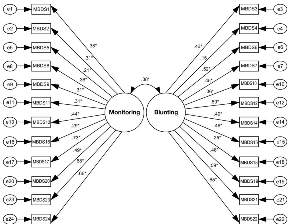
Figure 2. Path diagram for the MBDS two factor model with completely standardized parameter estimates.
