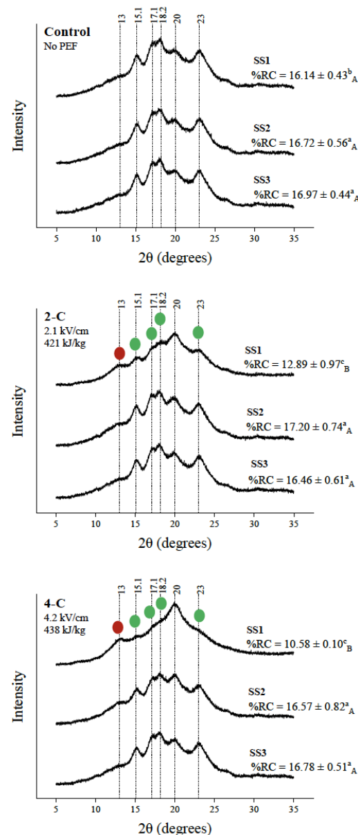
Figure 6. X-ray diffractograms and percent relative crystallinity (%RC) of flour segments collected from PEF-treated oat flour at 418–484 kJ/kg. The %RC values are displayed as mean \pm standard error of mean ( n = 3 , collected and pooled from 24–34 independent samples). Means sharing the same lowercase letters in superscript indicate no significant difference ( p < 0.05 ) between treatments obtained from the same segment (e.g., 2-C, SS1 vs. SS2 vs. SS3). Means sharing the same uppercase letters in subscript indicate no significant difference ( p < 0.05 ) between flour segments obtained from different treatments (e.g., SS1, Control vs. 2-C vs. 4-C). Green dots direct to the modification of specific peaks due to PEF treatment. Red dots highlight the new peaks observed in flour segments collected from PEF-treated oat flour.
