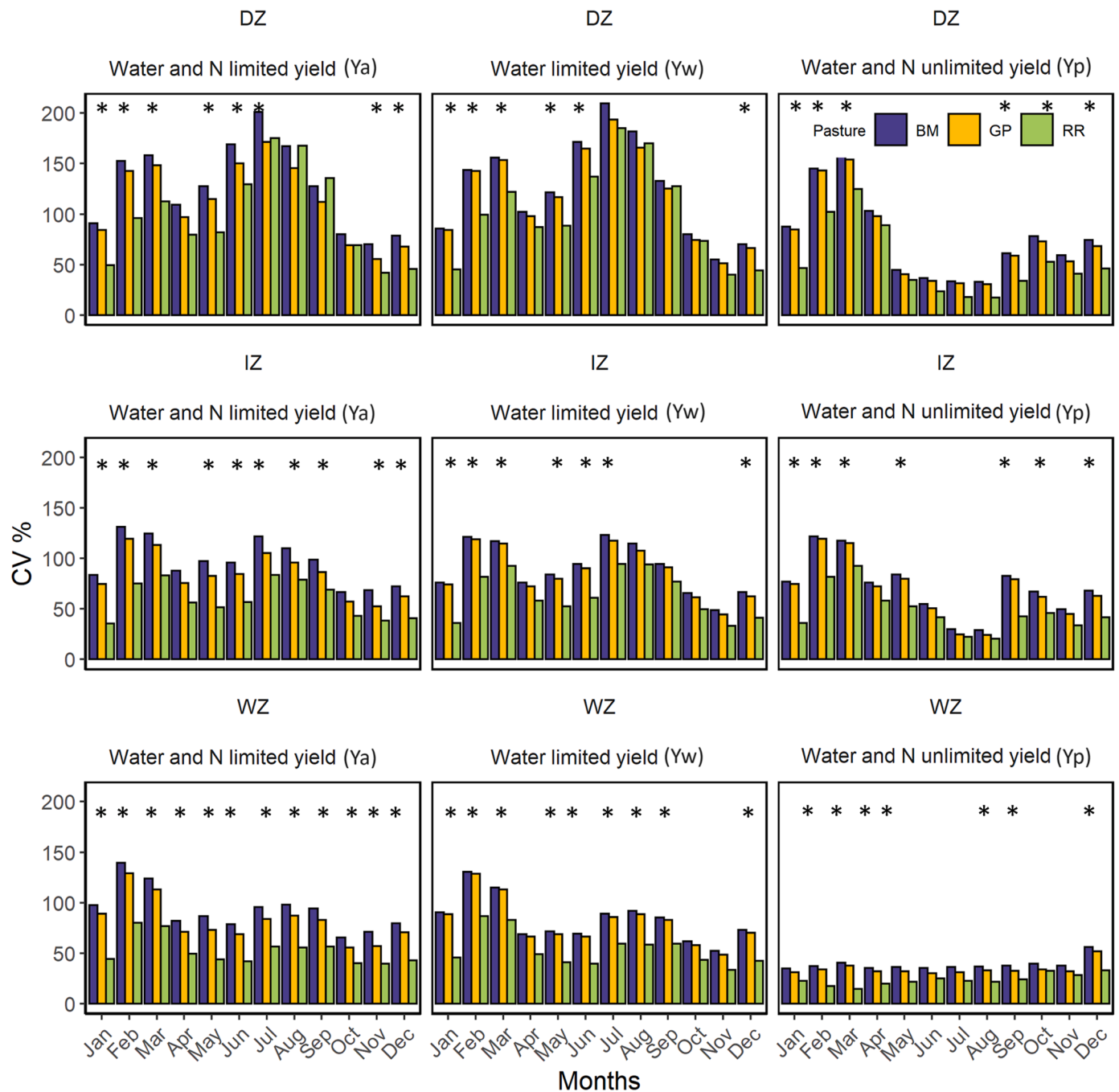
Fig. 4. Long-term interannual variability (CV %) of monthly pasture growth of Brachiaria Mulato II (BM), Gattton panic (GP), and Rhodes grass Reclaimer (RR) for the locations in three major climatic zones (DZ = dry zone, IZ = intermediate zone, WZ = wet zone) under different pasture management scenarios in Sri Lanka. *Statistically significant at p < 0.05 within each month.
