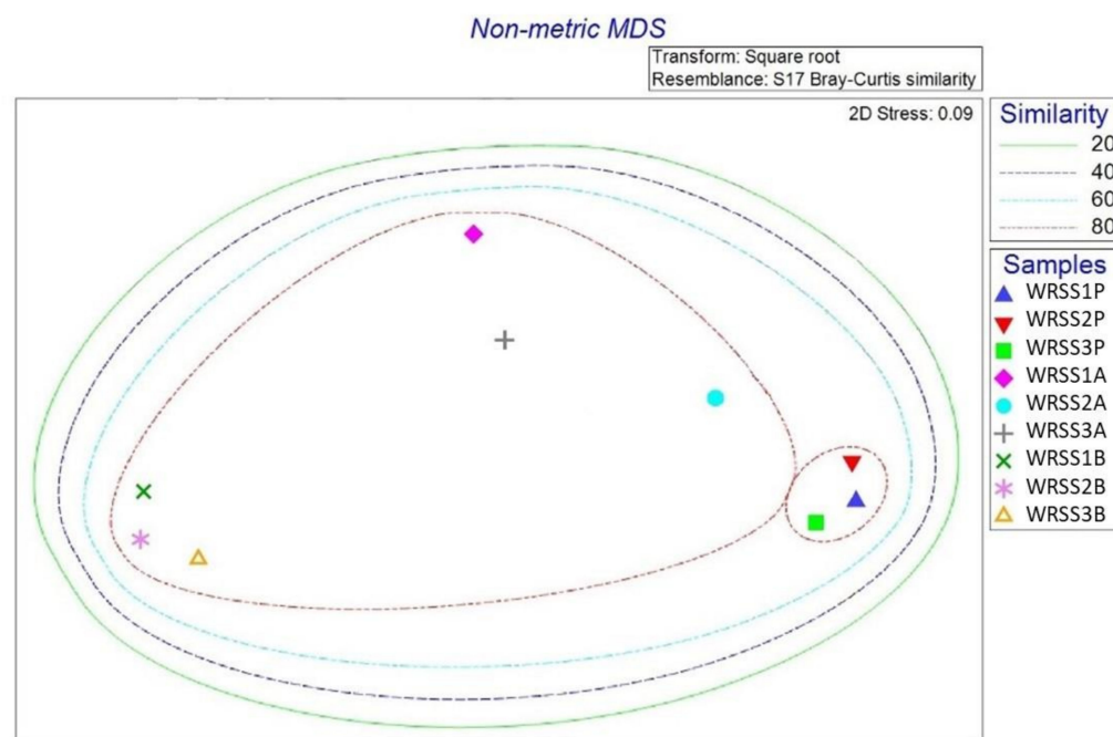
Figure 8. Non-metric multidimensional scaling analysis plot of TRFLP relative peak height for WR soils' bacterial communities' data, using the Bray-Curtis similarity index. Significant difference ( p < 0.05 ) between the two clusters characterised with >80\% of similarity.
