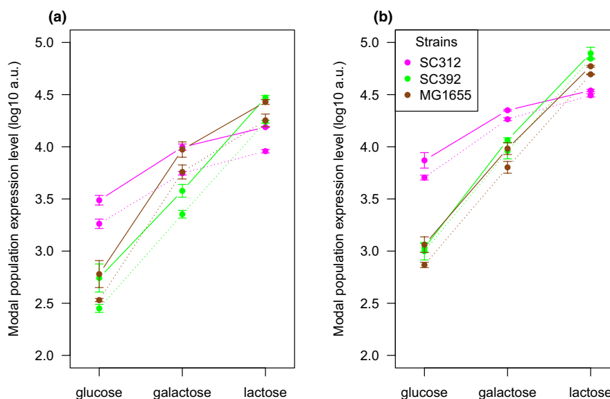
FIGURE 1 Modal expression levels differ consistently due to a single A to C change at position +69 of the lacZ open reading frame both without RiboJ (a) and with RiboJ (b) and across genetic backgrounds. Shown are the modal population fluorescence levels for GFP driven by an upstream lacZ promoter for three divergent strains of E. coli . In all genetic backgrounds tested and all growth conditions (glucose, galactose, and lactose), the fluorescence levels from a promoter with the 69C polymorphism (dotted line) were consistently lower than those from the promoter with the 69A polymorphism (solid line). On the log 10 scale that is shown, a 0.1 difference is equivalent to a 25% change in expression. There are clear effects of genetic background on both the level and dynamic range of protein expression. In particular, SC312 has a narrow dynamic range, with relatively high expression in non-lactose environments compared to the other strains, but relatively low expression in lactose. Despite this, the effect of the A to C change is nearly constant. Whiskers show one standard deviation of three replicates
