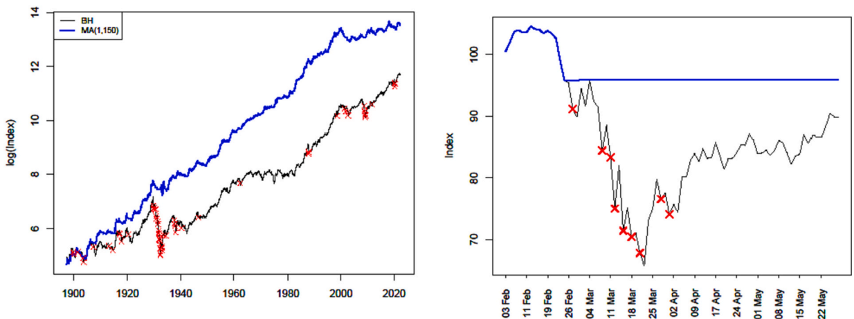
Fig. 1. Buy-and-hold vs MA(1150). These figures show the performance of a BH strategy (thin black line) and the TTR MA(1150) rule (thick blue line) for the DJIA. The ability of the
