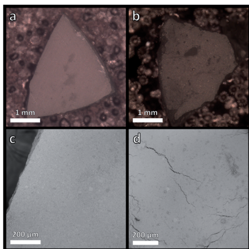
Fig. 3 Optical images of (a) (MIL-118) 0.5 (a g ZIF-62) 0.5 , and (b) (UL-MOF-1) 0.5 (a g ZIF-62) 0.5 , and scanning electron microscopy images taken of a fragment of (c) (MIL-118) 0.5 (a g ZIF-62) 0.5 , and (d) (UL-MOF-1) 0.5 (a g ZIF-62) 0.5 .
