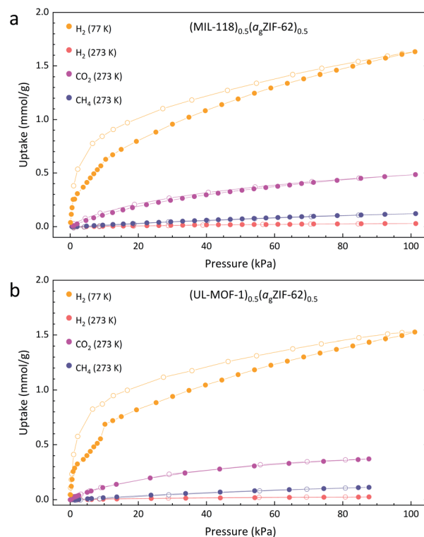
Fig. 5 Gas adsorption isotherms of samples of (a) (MIL-118) 0.5 (a g ZIF-62) 0.5 and (b) (UL-MOF-1) 0.5 (a g ZIF-62) 0.5 . Solid and open circles of the same colour indicate the adsorption and desorption respectively.
