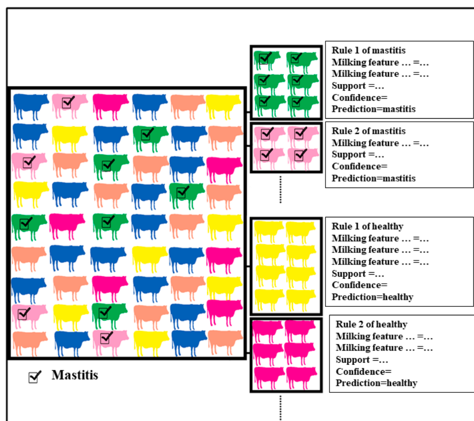
Figure 2. Classification based on associations is a high performing and robust classifier that integrates the classification algorithm with the association rule mining algorithm to deal with data heterogeneity. Classification based on associations finds homogenous groups within heterogenous data, based on minimum support. Then, classifier applies discriminative rules with high confidence in each homogenous group.
