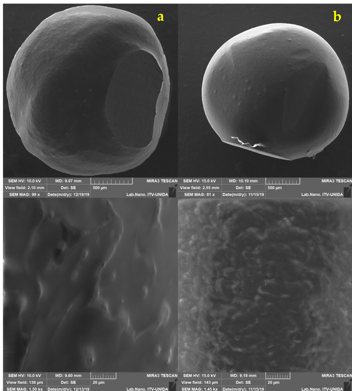
Figure 2. Micrographs from scanning electron microscopy of the LG alginate (ALG) systems made by ALG AM magnetic stirring (column (a)), rotor-stator ALG UT (column (b)) drip homogenization.
