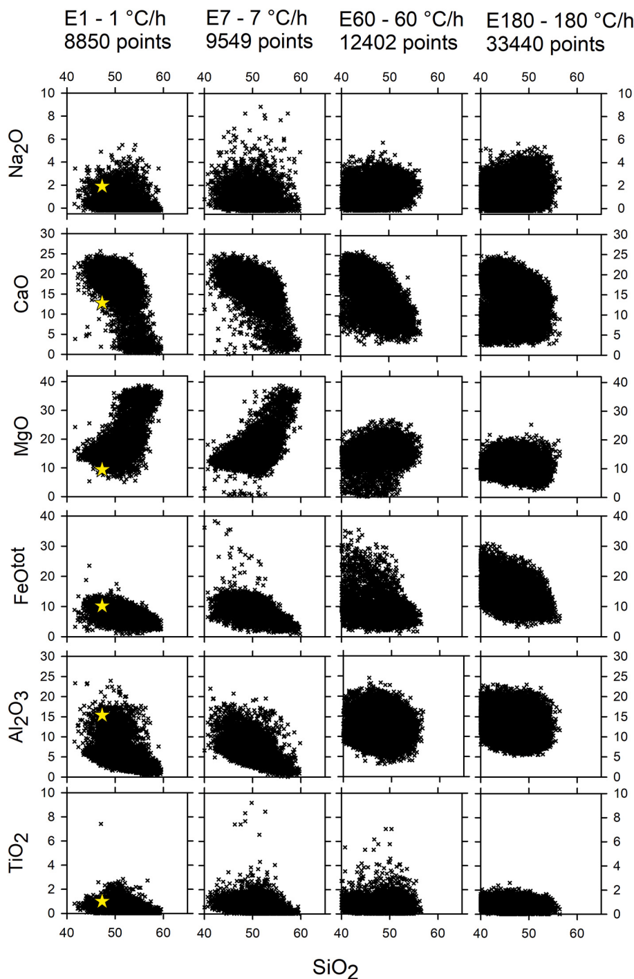
Fig. 1. Chemical variations of major oxides (wt%) in px as a function of SiO 2 content and \Delta T/\Delta t . Yellow star (left column) is the starting B 100 melt composition. (For interpretation of the references to colour in this figure legend, the reader is referred to the web version of this article.)
