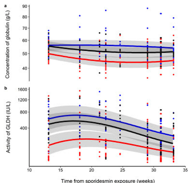
Figure 3. Fitted curves with 95% CI (light grey shading) from linear mixed effects models describing the change over time of (a) the concentration of globulin and (b) the activity of glutamate dehydrogenase (GLDH) in serum of ewes ( n = 46 ) exposed to acute sporidesmin toxicity ending in late April 2019 (week 0) categorised by liver disease category (LDC; red = low LDC, black = middle LDC; blue = high LDC). Note the square root scale of the y-axis.
