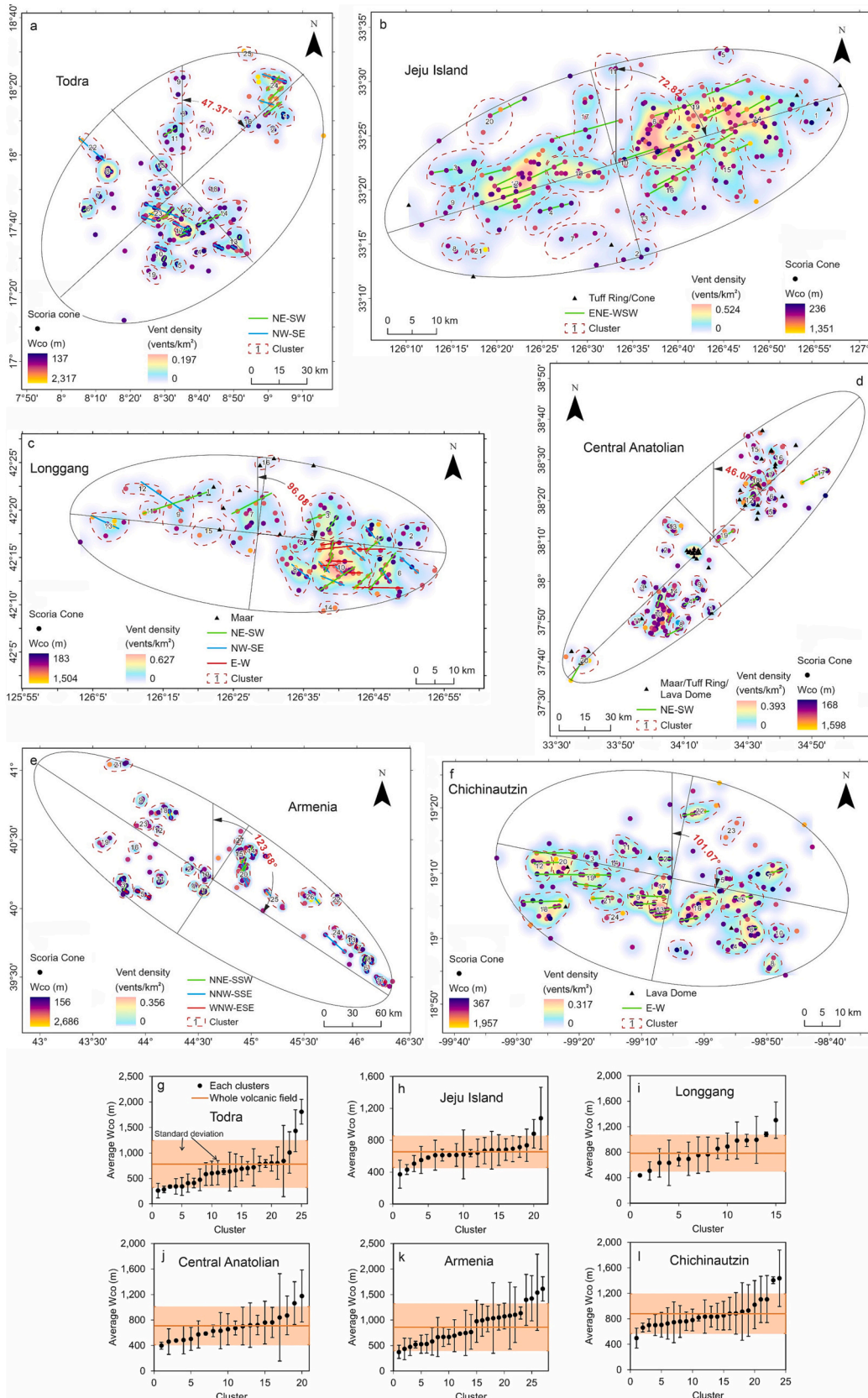
Fig. 8. (a–f) Minimum ellipse, scoria cone volume distribution, vent cluster and alignment of selected volcanic fields. Ellipses mark the calculated minimum ellipses of each volcanic field. Red numbers indicate the angles of the long axes of the ellipses. Vent alignments of each volcanic field are summarized by the methods of Lutz (1986) and Cebriá et al. (2011) as well as previous studies (e.g., Le Corvec et al., 2013; Zhao et al., 2021). (g–l) Comparison of the average Wco of individual clusters and the overall average Wco of each volcanic field. Wco = Cone base width.
