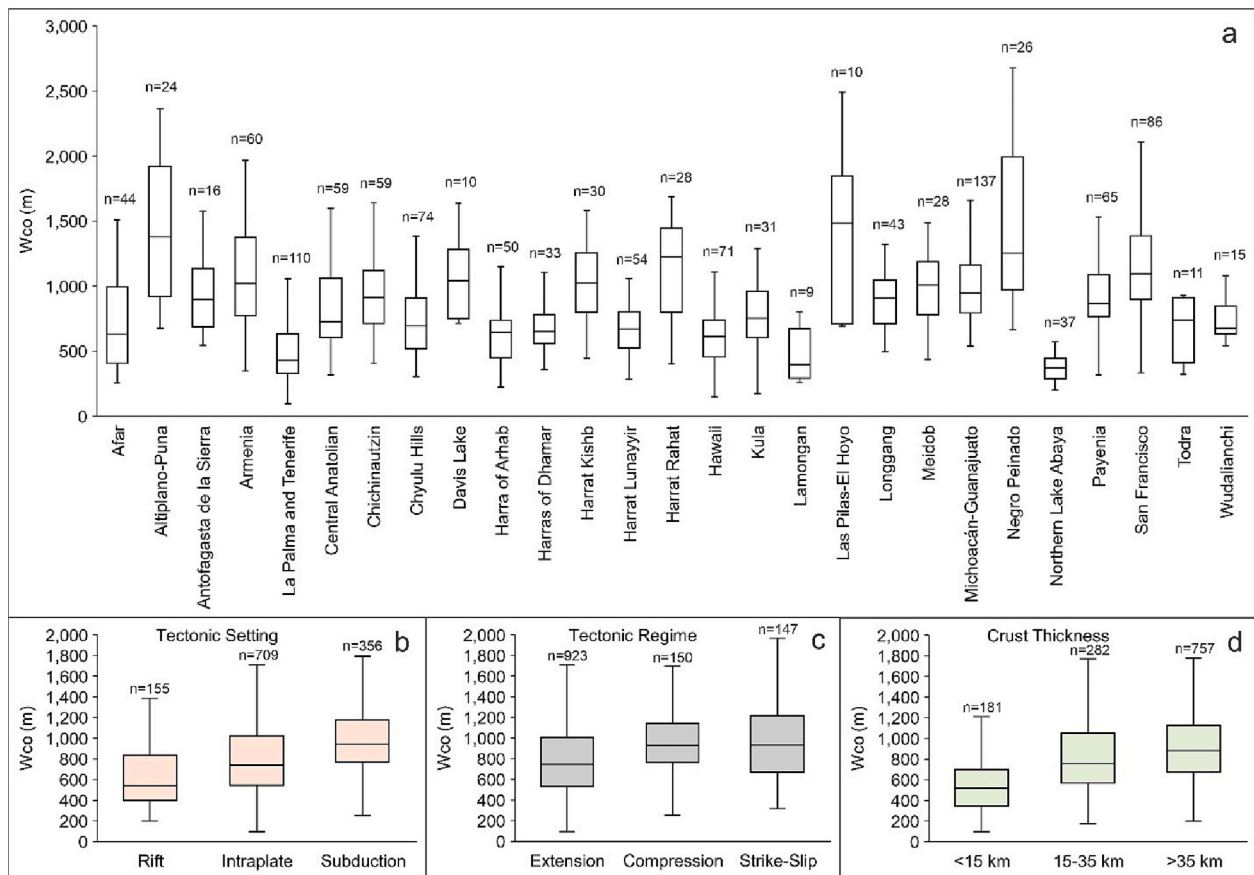
Fig. 5. (a) Boxplot of Wco in the selected 27 volcanic fields. (b) Boxplot of Wco by tectonic setting. (c) Boxplot of Wco by tectonic regime. (d) Boxplot of Wco by crust thickness. Wco = Cone base width.
