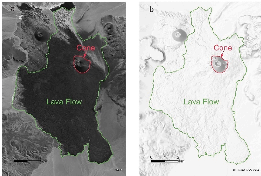
Fig. 1. Cone and lava flow of Alumbreira volcano (Antofagasta de la Sierra Volcanic Field, Argentina) delineated on Maxar satellite image (a), and shaded terrain models from Esri/NASA/NGA/USGS (b).
