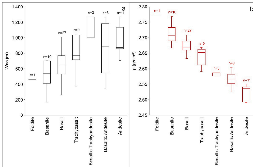
Fig. 7. Boxplots of the relationship between rock type and Wco (a), and between rock type and magma density (b). Wco = Cone base width.
