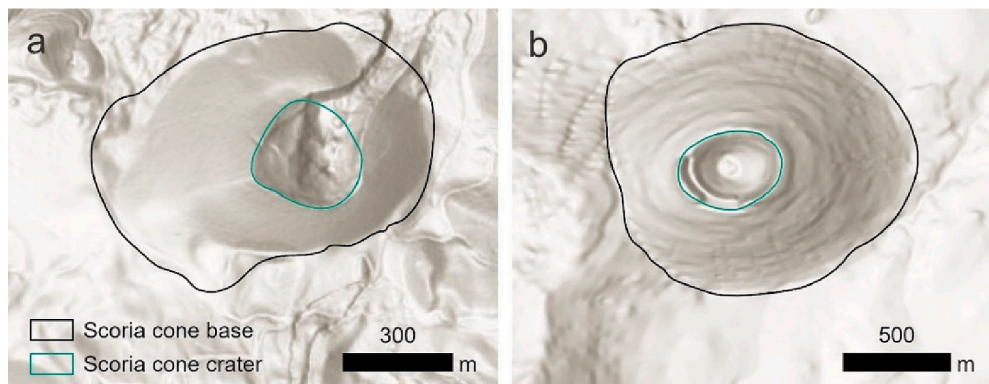
Fig. 2. Classification examples of breached scoria cone (Montana Quemada, La Palma, Canary Islands) (a) and intact scoria cone (SP Crater, San Francisco Volcanic Field, United States) (b). Terrain maps from Esri, NASA, NGA, USGS.
