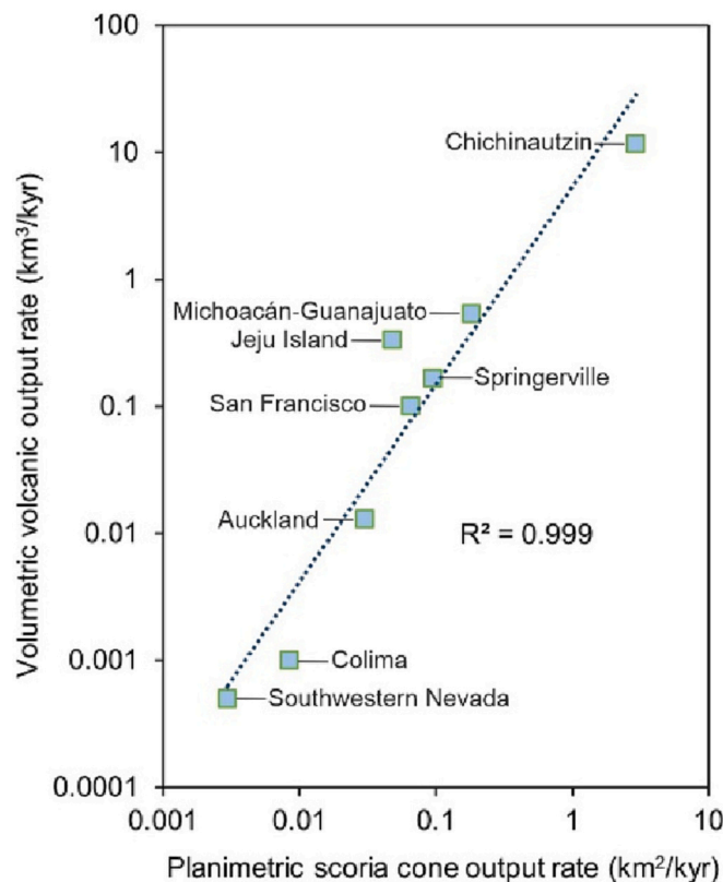
Fig. 10. Comparison between planimetric scoria cone output rate and volumetric volcanic output rate. Note the log-log scale. The blue dash line is a power trend line. (For interpretation of the references to colour in this figure legend, the reader is referred to the web version of this article.)
