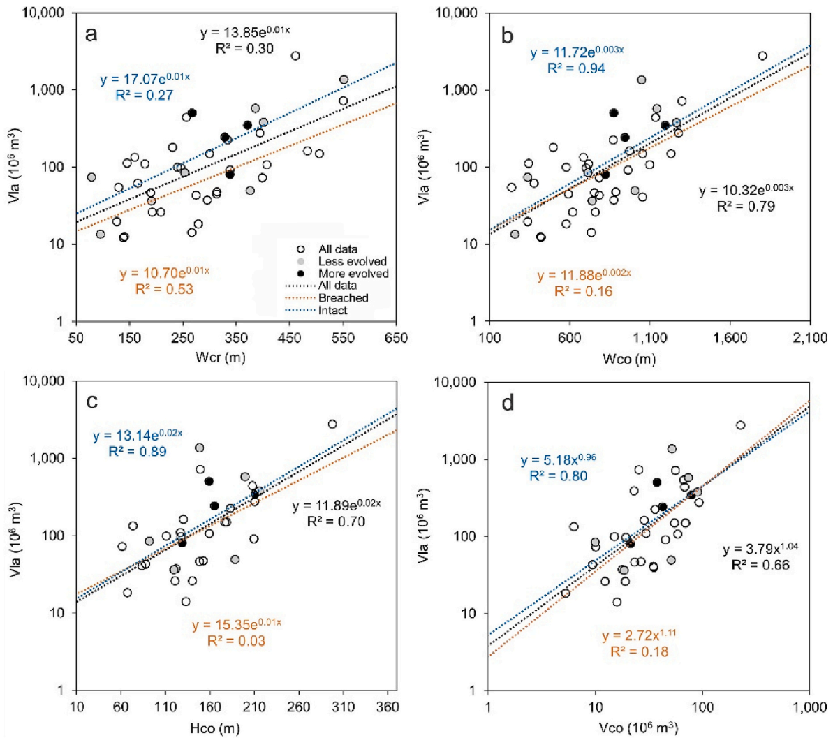
Fig. 4. Scatter plots of cone morphometry vs. associated lava flow volume. (a–c) Plots of Wcr , Wco and Hco vs. Vla . Dash lines are exponential trend lines. (d) Plots of Vco vs. Vla . Black, orange and blue dash lines are power trend lines of all data, breached and intact cones, respectively. Vco = Cone volume, Vla = Lava flow volume, Wcr = Crater width, Hco = Cone height, and Wco = Cone base width. (For interpretation of the references to colour in this figure legend, the reader is referred to the web version of this article.)
