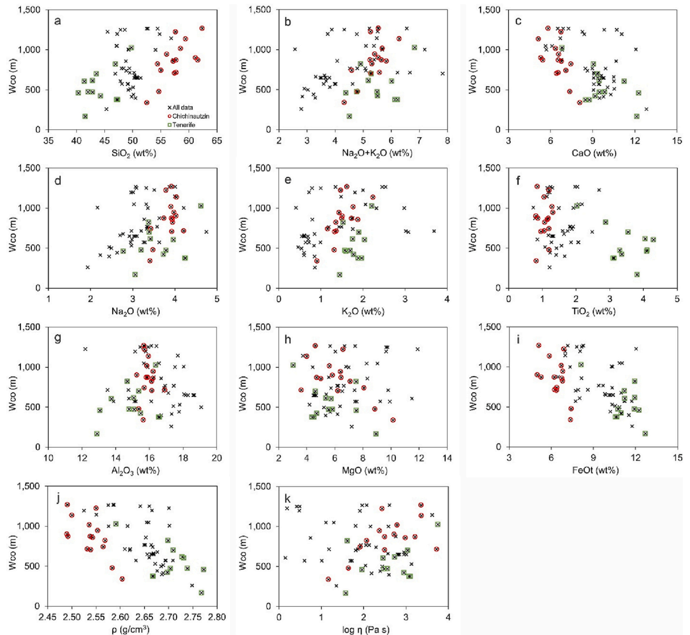
Fig. 6. X-Y plots of scoria cone chemical elements and physical parameters vs. Wco. Wco = Cone base width.
