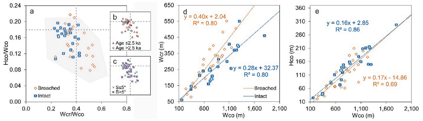
Fig. 3. (a) Plot of Hco/Wco vs. Wcr/Wco . Gray dash lines indicate the “ideal” cone values taken from Porter (1972) and Wood (1980). Gray area refers to the data from Fornaciai et al. (2012). (b–c) The inset shows the same graph as (a) but classified by age (b) and pre-eruptive surface inclination (c). (d) Plot of Wcr vs. Wco . (e) Plot of Hco vs. Wco . Orange and blue dash lines refer to linear trend lines for breached and intact scoria cones, respectively. Wcr = Crater width, Hco = Cone height, Wco = Cone base width, and S = Slope angle of pre-eruption surface. (For interpretation of the references to colour in this figure legend, the reader is referred to the web version of this article.)
