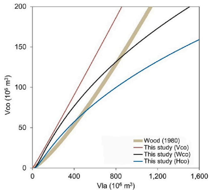
Fig. 9. Comparison of different volume relationships between scoria cones and associated lava flows. V_{co} derived from W_{co} and H_{co} , respectively, is calculated according to eq. (2) of Riedel et al. (2003), which assumes cones have reached the angle of repose and H_{co}/W_{co} and W_{cr}/W_{co} are the ideal values proposed by Porter (1972) and Wood (1980). V_{la} derived from W_{co} and H_{co} is based on Eq. 7 and Eq. 8, respectively. The red line is the relationship between V_{co} and V_{la} for the intact cones in Fig. 4d. V_{co} = Cone volume, V_{la} = Lava flow volume, H_{co} = Cone height, and W_{co} = Cone base width. (For interpretation of the references to colour in this figure legend, the reader is referred to the web version of this article.)
