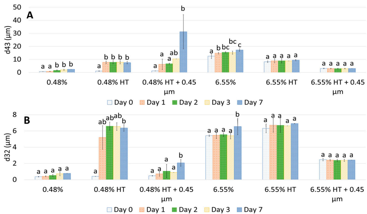
Figure 4. Changes in d_{43} (A) and d_{32} (B) over 7 days of storage of 10% oil-in-water emulsions made with unmodified, heat-treated (HT), and heat-treated + filtrated (HT + 0.45 \mu\text{m} ) GWSC extracts (0.48% and 6.55% wt/wt). A different statistical analysis was applied for each concentration. Samples within the concentration and treatment groups with the same letter(s) did not present significant differences ( p > 0.05 ).
