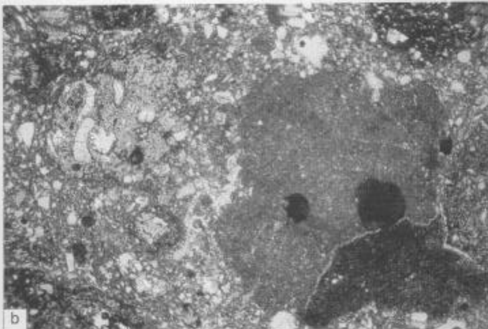
Fig. 2a, b Photomicrographs of the PXLt lithofacies from locality D (see Fig. 1). In both pictures the shorter side of the picture is 2 mm. Note the bright, white-colored, small, angular fragments. They are quartz fragments derived from the Pannonian clastic deposits. In Fig. 2a note the difference between sideromelane (small, microvesiculated, slightly rounded, elongate lighter colored shard in the top/left corner) and tachylite glass shards (large, angular black fragment in the middle of the picture)
