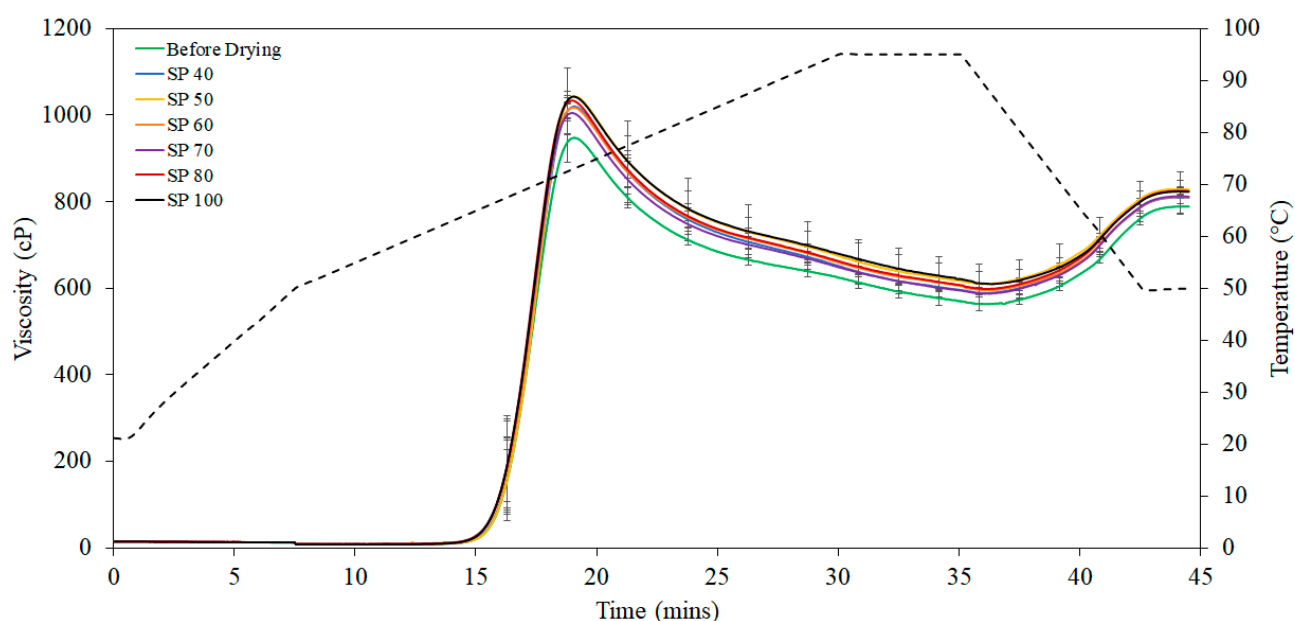
Figure 2. Pasting profile of native and spray dried waxy rice starches.
