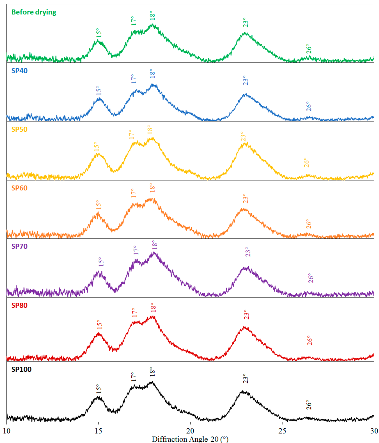
Figure 4. X-ray diffractograms (XRD) of native (Before Drying) and spray dried waxy rice starches.
