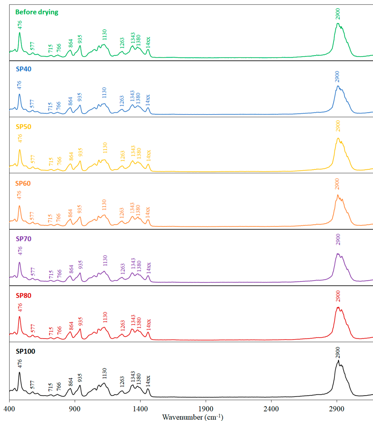
Figure 5. Raman spectra of native (Before Drying) and spray dried waxy rice starches.
