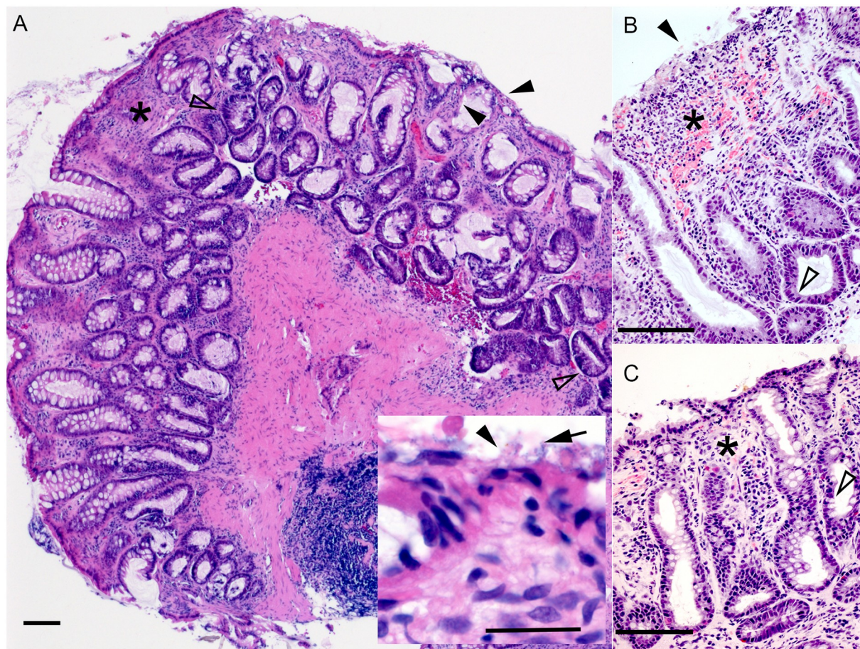
Fig 2. Colonic histopathology, proximal colon, dogs with AHDS. (A) FMT-recipient dog from New Zealand. H&E, bar = 100 µm. Inset, H&E, bar = 25µm. (B & C) FMT-recipient and sham-control dogs from South Africa. H&E, bar = 100 µm. Black arrowhead: denuded ulcerated colonic mucosa; Black arrow: denuded mucosa with adherent colonic bacteria; Black asterisk: leukocytes, admixed with hemorrhage and edema infiltrate the colonic lamina propria. The latter has loss of colonic glands with collapse of the supporting stroma; Open arrowhead: 1–2 layers of large hyperchromatic colonic epithelial cells pile up and exhibit frequent mitoses (regeneration).
