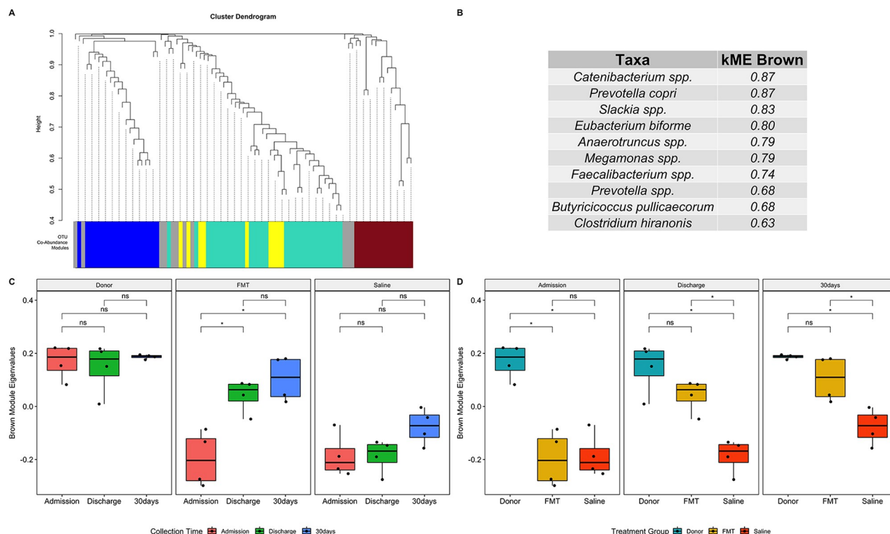
Fig 8. Weighted co-abundance analysis identified a subnetwork of bacteria significantly associated with FMT. A weighted co-abundance network was generated to identify subnetworks (modules) of taxa associated with FMT. Module eigen-OTUs (a mathematical summary of module abundance derived from principal component analysis) were used to detect differences in module abundance among treatment groups and collection times. (A) A cluster dendrogram of OTUs with correlated patterns of abundance. The OTUs were grouped into 6 modules and represented by an arbitrarily unique color below the dendrogram. OTUs that were not grouped into a co-abundance module are represented by the gray color. (B) The “Brown” module was found to contain the same taxa that were differentially abundant in post-FMT samples. The importance of each OTU within the “Brown” module was quantified by the module eigen-OTU connectivity (kME), also known as module membership. As the kME of a given OTU approaches 1, it more closely characterizes the abundance pattern of the whole module. OTUs with kME > 0.5 are shown. (C) The “Brown” module was increased at discharge and 30 days in FMT recipients but was unchanged in sham-treated controls. (D) “Brown” module abundance was decreased in the FMT and sham-treated control groups at admission. The “Brown” module increased in abundance in FMT recipients at discharge and 30 days, compared with sham-treated controls. There were no statistically significant differences in “Brown” module abundance between donors and FMT-recipients at discharge or 30 days. Statistical comparisons among treatment groups and collection times are indicated by annotated brackets where “ns” represents P \geq 0.05 and “*” represents 0.01 < P < 0.05 . FMT: fecal microbial transplantation.
