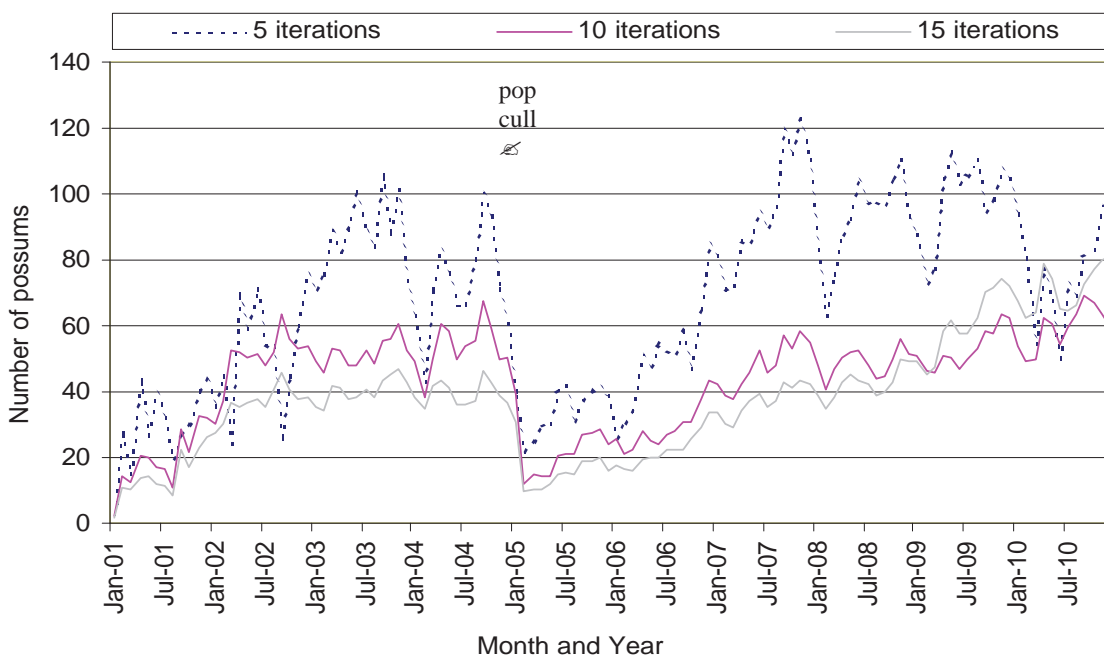
Figure 36. The 95% confidence interval range (Upper CI – lower CI) for the mean population each month using 5, 10 and 15 iterations for the high-density population.
