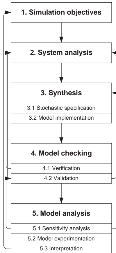
Figure 8. Five stage approach to model development (Adapted from: “Anderson, 1974)
