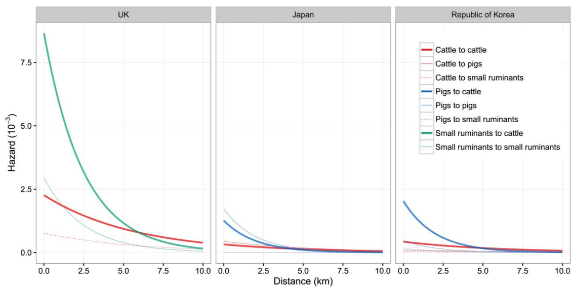
Figure 3-4 Predicted adjusted daily hazard of local spread of foot-and-mouth disease (FMD) on the first day of infectiousness for the FMD outbreak in Cumbria (UK, 2001), Miyazaki (Japan, 2010) and Andong (Republic of Korea, 2010).
