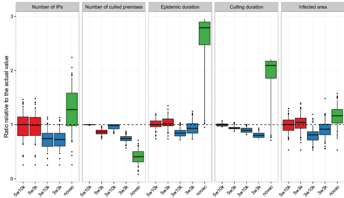
Figure 4-7 Box and whisker plots showing the ratios of the simulated outcomes of an epidemic for the number of infected premises (IPs, reference: 280 IPs), the number of culled (infected or vaccinated) premises (880 premises), epidemic duration (57 days), culling duration (76 days) and the size of the infected area (187 km 2 ) to the actual values (in parenthesis) for the five control strategies (5w10k, 5w3k, 3w10k, 3w3k and novac: 10 km vaccination in week 5, 3 km vaccination in week 5, 10 km vaccination in week 3, 3 km vaccination in week 3 and no vaccination) for the foot-and-mouth disease (FMD) epidemic in Japan (2010). The box, whisker, and dot represent the interquartile range (IQR), 5 th and 95 th percentile, and outliers, respectively.
