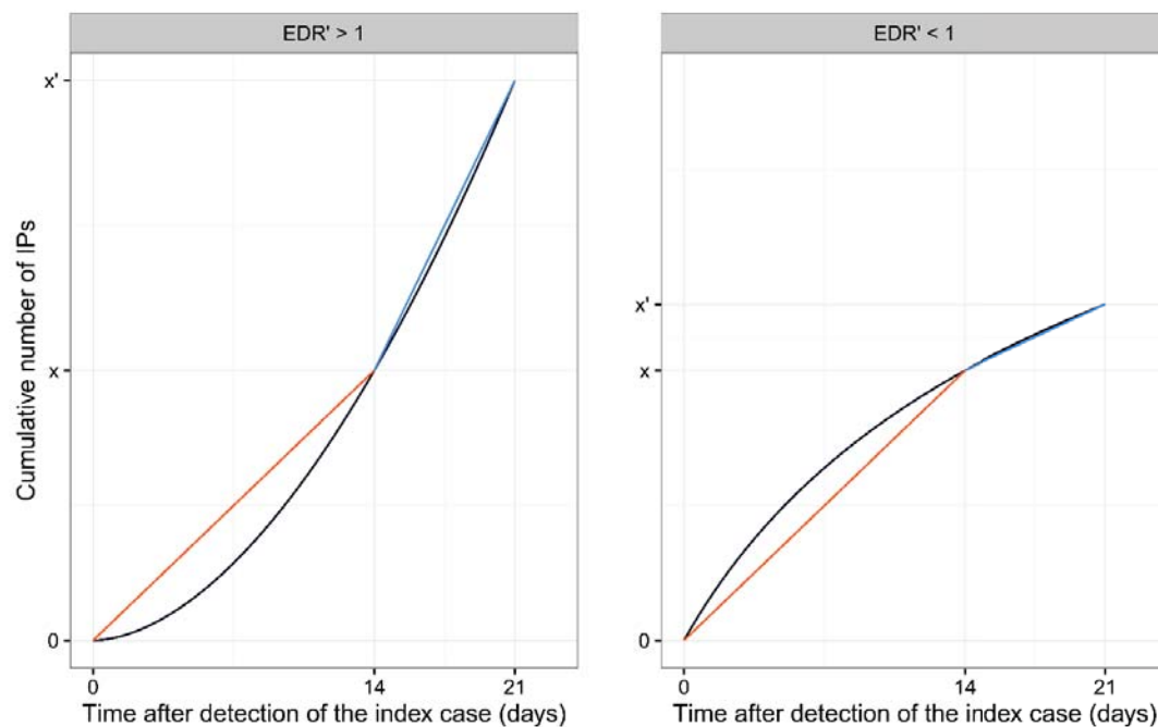
Figure 6-2 Cumulative epidemic curves with a crude estimated dissemination rate ( EDR' ) greater than 1 [left] and smaller than 1 [right], representing a growing epidemic and a diminishing epidemic. EDR' is calculated as the slope of line between days 14 and 21 (blue) divided by that of days 0 and 14 (orange).
