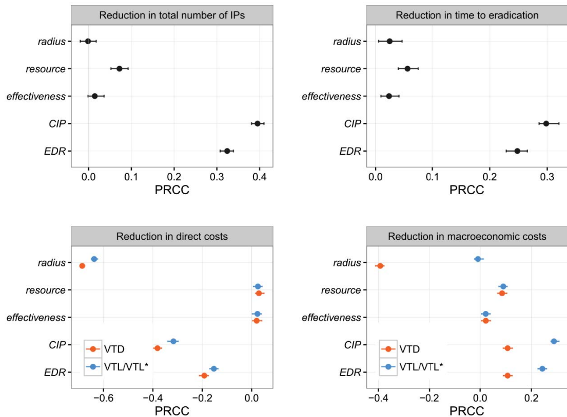
Figure 7-2 Partial rank correlation coefficients (PRCC) for varied explanatory variables: vaccination radius ( radius , 1 – 20 km), resource capacity ( resource , 100 – 500 premises/day), effectiveness of vaccination ( effectiveness , 75% - 100%), cumulative number of IPs ( CIP ) and estimated dissemination rate ( EDR ) for four outcome variables for 21 st -day start vaccinate-to-die (VTD), vaccinate-to-live (VTL), and vaccinate-to-live with a 3-month waiting period (VTL*) for control of a simulated foot-and-mouth (FMD) disease epidemic in Auckland Region (n = 13,459).
