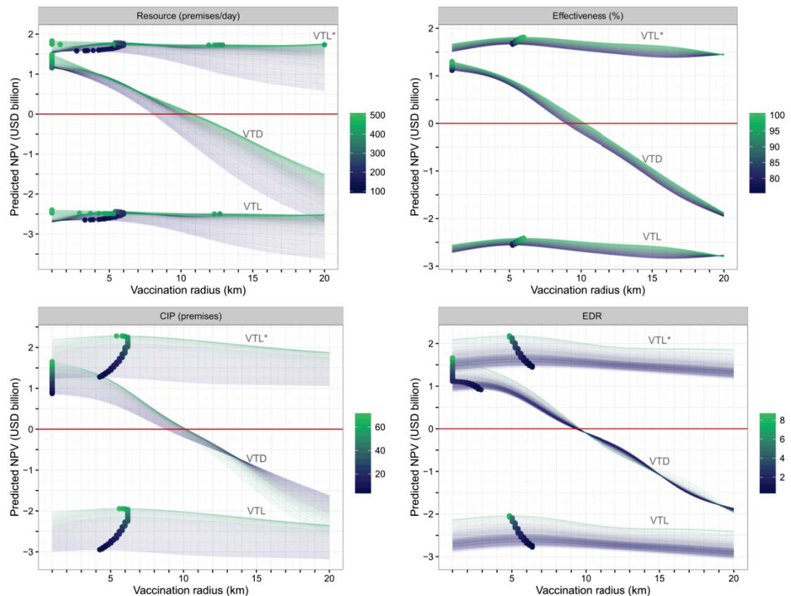
Figure 7-3 Predicted net present values (NPVs) of simulated foot-and-mouth disease (FMD) epidemics in the Auckland Region controlled by vaccinate-to-die (VTD), vaccinate-to-live (VTL), and VTL of a shortened waiting period (VTL*) relative to stamping-out alone, with varying vaccination radii, adjusted for resource capacity, effectiveness of vaccination, cumulative number of IPs (CIP) and estimated dissemination rate (EDR).
