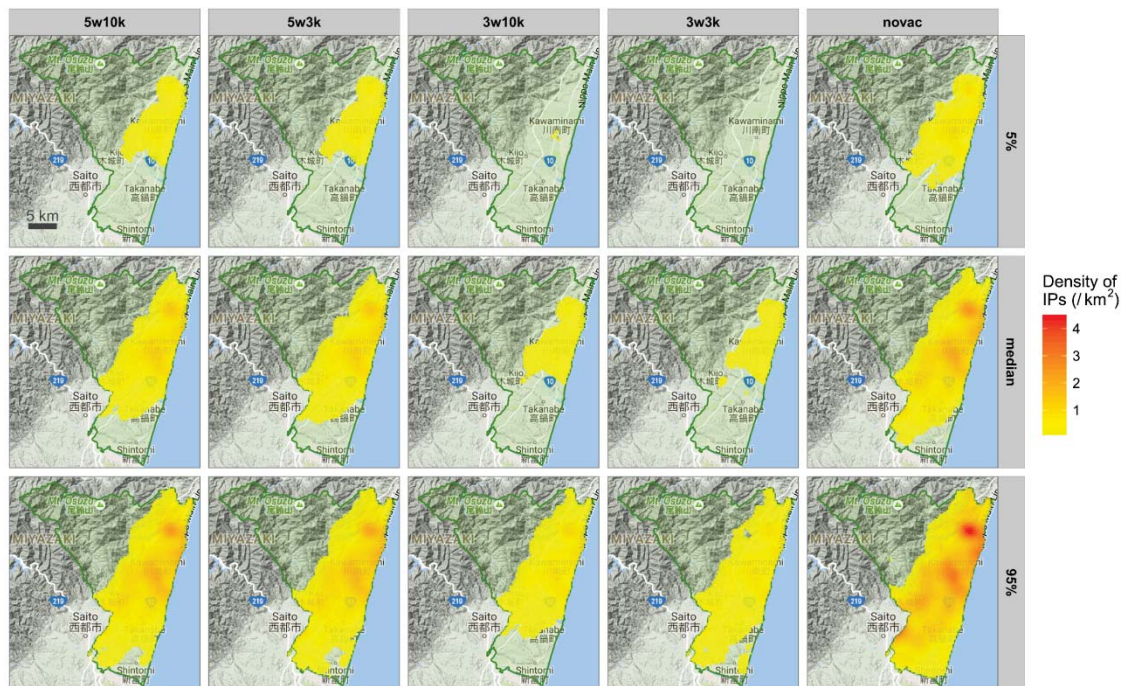
Figure 4-8 Kernel density (bandwidth = 1.00 km) of simulated cases (median, 5 th and 95 th percentiles of 100 iterations), infected after 21 days onwards since the first confirmation of disease, controlled by the actual (5w10k: 10 km vaccination in week 5) and four alternative strategies (5w3k: 3 km vaccination in week 5, 3w10k: 10 km vaccination in week 3, 3w3k: 3 km vaccination in week 3, novac: no vaccination) for the foot-and-mouth disease (FMD) epidemic in Japan (2010).
