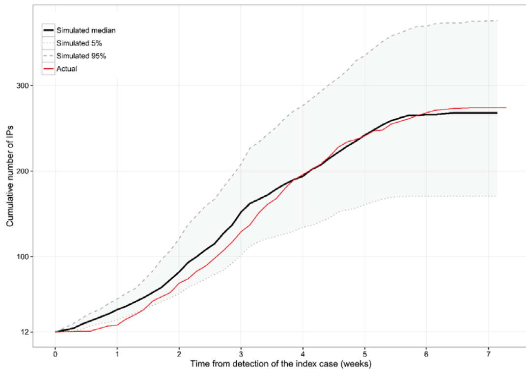
Figure 4-4 Cumulative number of infected premises (IPs) for the actual and simulated epidemics (median and the 5 th and 95 th percentiles of 100 iterations) for the foot-and-mouth disease (FMD) epidemic in Japan (2010).
