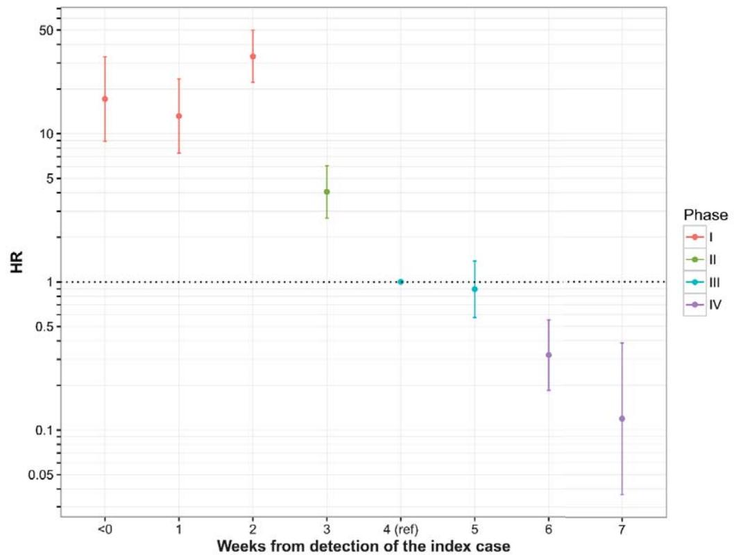
Figure 4-2 Estimated hazard ratio (HR) (points) and 95% confidence intervals (whiskers) of local spread of foot-and-mouth disease (FMD) for seven phases (silent spread phase, and weeks 1, 2, 3, 5, 6, and 7) relative to week 4, i.e., a week prior to application of vaccination (HR = 1: dashed line), for the FMD epidemic in Japan (2010).
