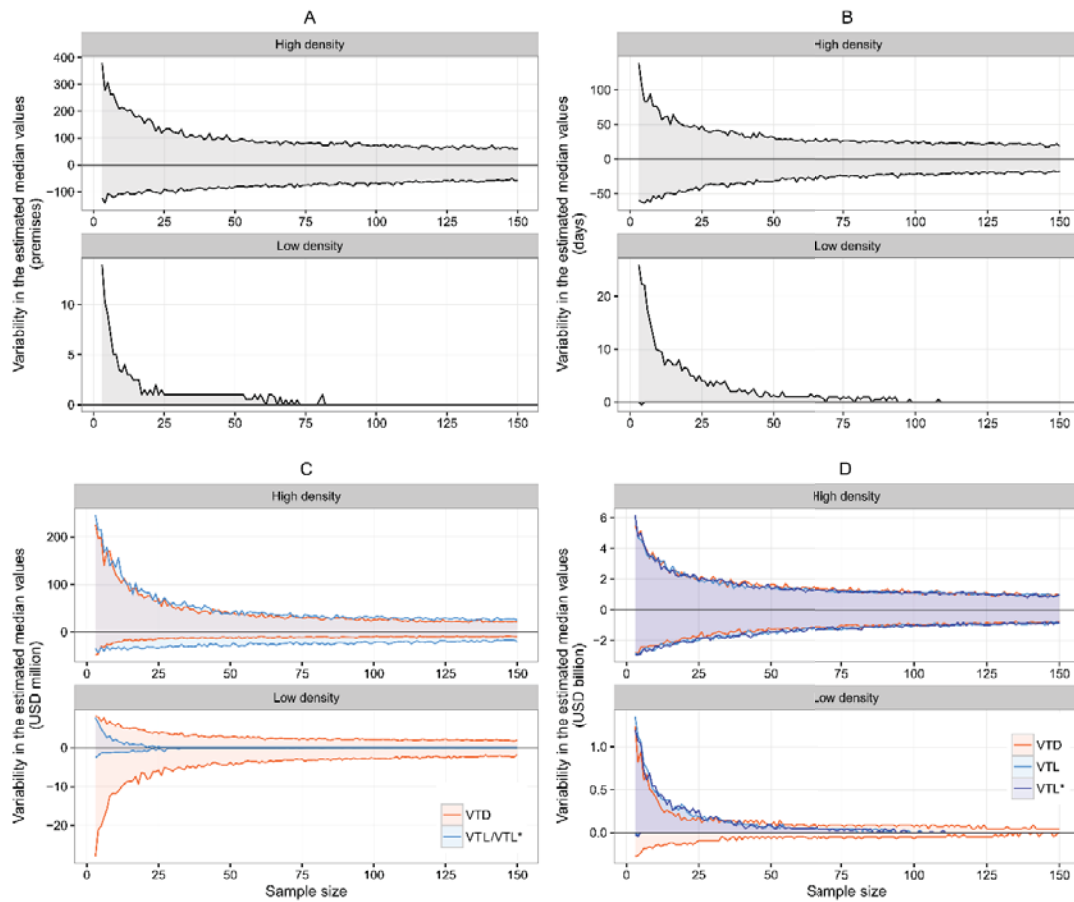
Figure 6-4 Variability in the estimated median values, measured by upper/lower 95% confidence limits minus median, for varying sizes of bootstrap samples, for simulated four outcome variables: reduction in the total number of infected premises (IPs) [A], time to eradication [B], direct costs [C] and macroeconomic costs [D] by region (high/low density) and control policy (vaccinate-to-die: VTD and vaccinate-to-live: VTL and VTL*).
