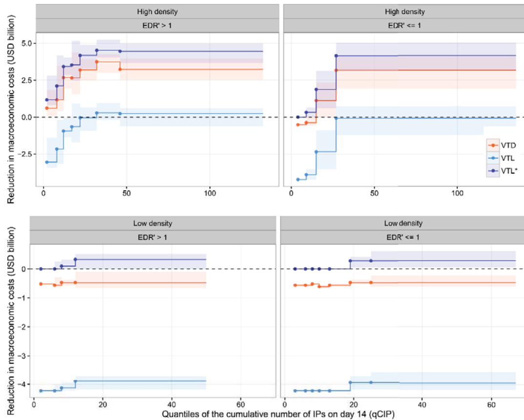
Figure 6-7 Effectiveness of vaccination policy (vaccinate-to-die: VTD and vaccinate-to-live with or without an additional 3-month waiting period: VTL/VTL*, all applied within 3 km on day 21 onwards after detection of the primary case) in reduction of the macroeconomic costs, presented as bootstrap median values (points) with their 95% CI (shade) by the region of incursion ( region ), estimated dissemination rate \leq 1 or > 1 ( EDR' ) and the lower limits of the quantiles of the cumulative number of infected premises (IPs) on day 14 ( qCIP ) for simulated foot-and-mouth disease (FMD) epidemics lasting for \geq 21 days in New Zealand ( n = 42 - 113 ).
