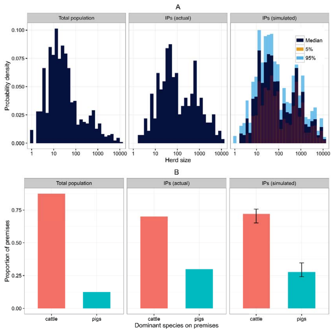
Figure 4-5 Distribution of herd size [A] and proportion of premises by dominant species on premises [B] for the total population, and actual and simulated infected premises (IPs) (median, 5 th and 95 th percentiles of 100 iterations) for the foot-and-mouth disease (FMD) epidemic in Japan (2010).
