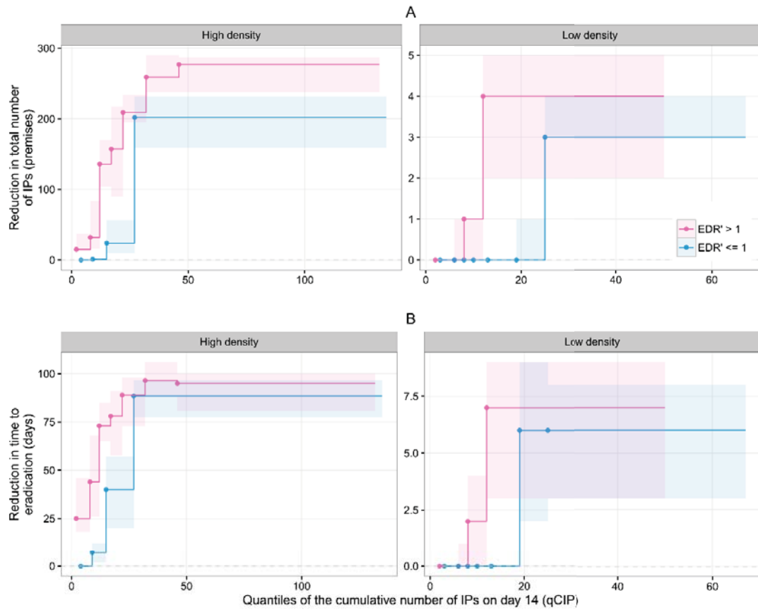
Figure 6-5 Effectiveness of vaccination policy (3-km ring vaccination starting on day 21 after detection of the primary case) in reduction of the total number of IPs [A] and time to eradication [B], presented as bootstrap median values (points) with their 95% CI (shade) by the region of incursion ( region ), estimated dissemination rate \leq 1 or > 1 ( EDR' ) and the lower limits of the quantiles of the cumulative number of infected premises (IPs) on day 14 ( qCIP ) for simulated foot-and-mouth disease (FMD) epidemics lasting for \geq 21 days in New Zealand ( n = 42 - 113 ).
