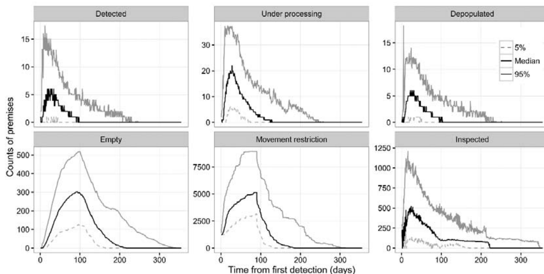
Figure 5-2 Median and the 5 th and the 95 th percentiles of the estimated number of premises where disease was detected, under processing, depopulated, empty (animals were absent), under movement restriction, and inspected, by time from the first detection for simulated foot-and-mouth disease (FMD) epidemics in Auckland, New Zealand (100 iterations).
