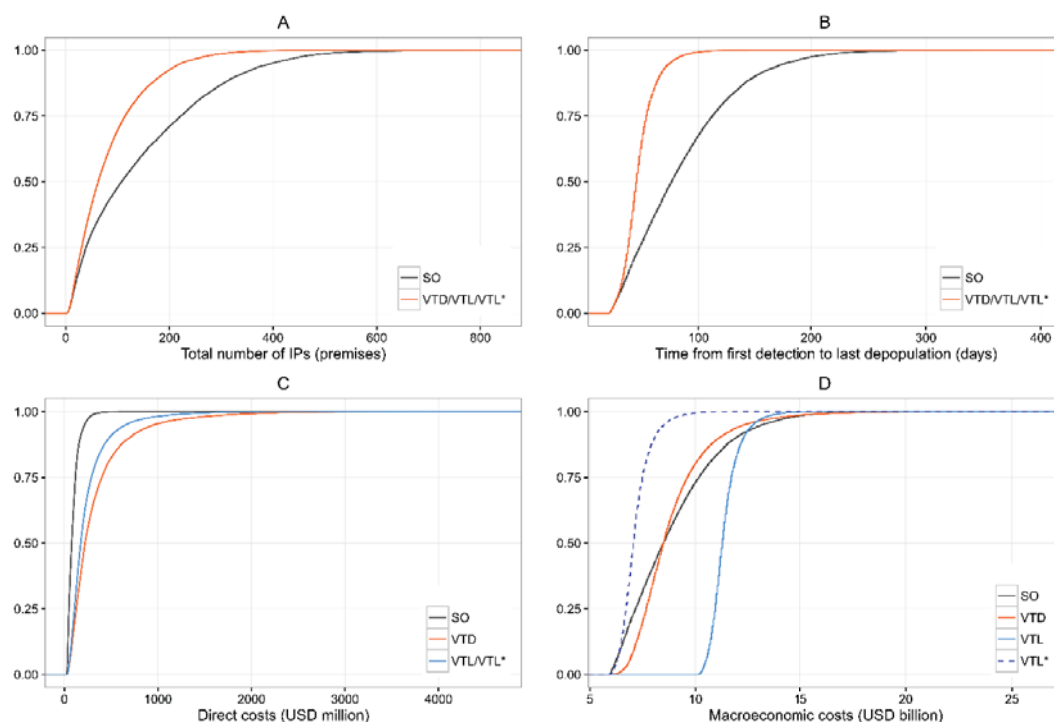
Figure 7-1 Cumulative distribution functions of the [A] total number of infected premises (IPs), [B] time till eradication, [C] direct costs and [D] macroeconomic costs for simulated foot-and-mouth disease (FMD) epidemics lasting for \geq 21 days in the Auckland Region, controlled by stamping-out (SO), vaccinate-to-die (VTD), vaccinate-to-live (VTL), and vaccinate-to-live with a 3-month waiting period (VTL*) ( n = 13,459 ).
