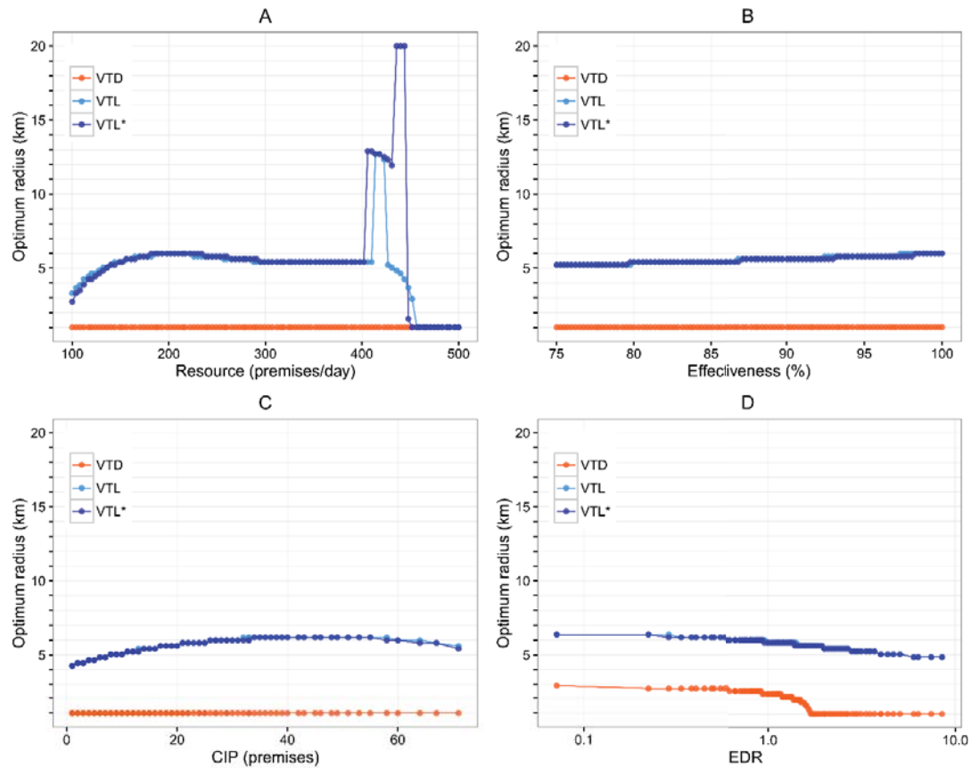
Figure 7-4 Optimal vaccination radius that minimised the predicted NPVs of vaccinate-to-die (VTD), vaccinate-to-live (VTL), and VTL of a shortened waiting period (VTL*) relative to stamping-out alone, while resource capacity [A], effectiveness of vaccination [B], cumulative number of IPs (CIP) [C] and estimated dissemination rate (EDR) [D] were varied to the quantiles of the designed or simulated values, for a simulated foot-and-mouth disease (FMD) epidemics in the Auckland Region.
