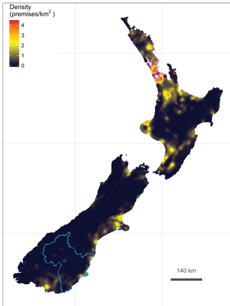
Figure 6-1 Kernel smoothed density of livestock premises (bandwidth = 5.0 km) susceptible to foot-and-mouth disease (FMD), and the location of Auckland (pink) and Otago (blue) regions, in which hypothetical primary cases were selected for FMD simulation.
