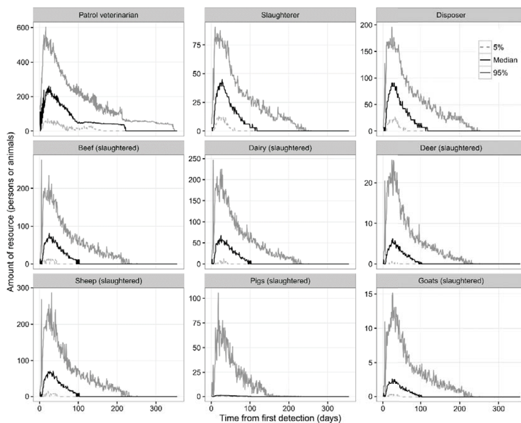
Figure 5-3 Median and the 5 th and the 95 th percentiles of the estimated amount of selected resources for calculation of the direct costs (variable costs of operation), for simulated foot-and-mouth disease (FMD) epidemics in Auckland, New Zealand (100 iterations).
