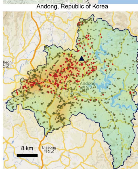
Figure 3-1 Location and infection status of all foot-and-mouth disease (FMD) susceptible livestock premises within the study area (blue triangle: primary case, red: infected, grey: uninfected) for the FMD outbreaks in Cumbria (UK, 2001), Miyazaki (Japan, 2010), and Andong (Republic of Korea, 2010).
