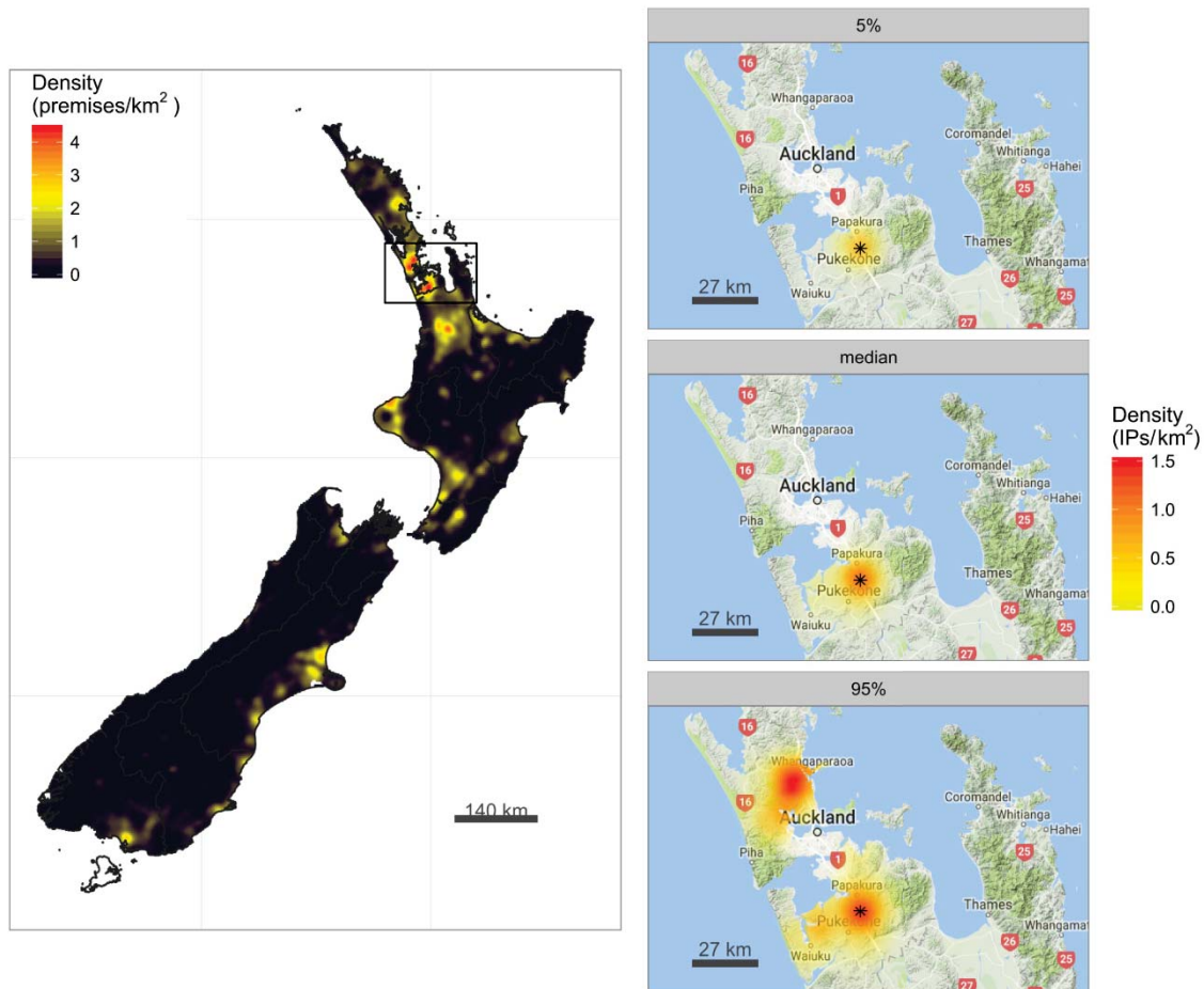
Figure 5-1 [Left] Map of New Zealand, showing the kernel smoothed density of livestock premises (bandwidth = 5.0 km). [B] Enlarged map of Auckland showing the kernel smoothed density of simulated IPs (median and the 5 th and the 95 th percentiles of 100 iterations, bandwidth = 5.0 km) and the location of the primary case (*).
