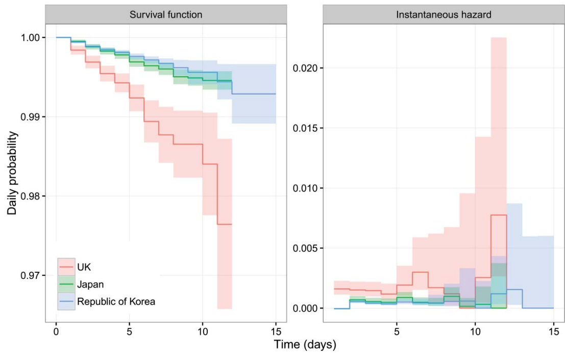
Figure 3-2 Survival function and instantaneous hazard estimated by Kaplan-Meier method (and 95% confidence intervals shown in shade) for local spread infection of foot-and-mouth disease (FMD) since the onset of infectiousness in the potential source premises for the FMD outbreaks in Cumbria (UK, 2001), Miyazaki (Japan, 2010), and Andong (Republic of Korea, 2010).
