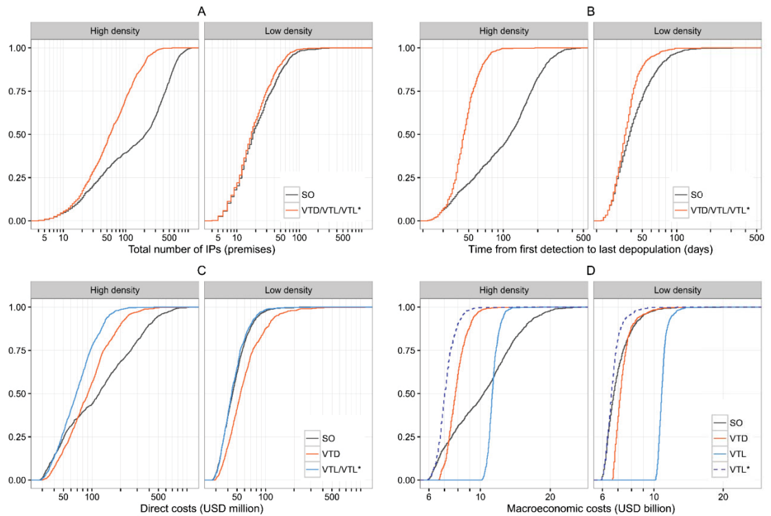
Figure 6-3 Cumulative distribution functions of the [A] total number of infected premises (IPs), [B] time till eradication, [C] direct costs and [D] macroeconomic costs for simulated foot-and-mouth disease (FMD) epidemics lasting for \geq 21 days in the high and low density regions in New Zealand, controlled by stamping-out (SO), vaccinate-to-die (VTD), vaccinate-to-live (VTL), and vaccinate-to-live with 3 month waiting period (VTL*) (1,013 and 822 iterations for high and low density regions).
