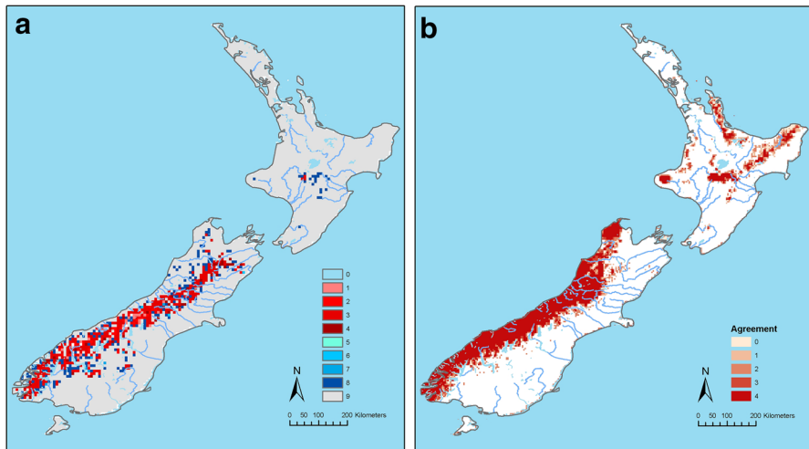
Fig. 4 a The agreement in predicted suitability of areas for Amblyomma americanum ticks between different Global Circulation Models (GCMs) under the High Emission, Representative Concentration Pathway (RCP) 8.5 emission scenario. Where 1=areas in which one of the four GCMs predicted suitability for A. americanum distribution. 2, 3, 4=two, three and four GCMs predicted suitability, respectively. 5=areas in which one of the four GCMs predicted loss of territory for A. americanum compared to the present-day distribution. 6, 7, 8=two, three, and four GCMs predicted loss of territory, respectively. 9=no observed change from predicted current distribution. b Degree of agreement between Global Circulation Models (GCMs) on extrapolative prediction of suitability areas for A. americanum ticks under the Low Emission, Representative Concentration Pathway (RCP) 4.5 Scenario. Where 1=Areas in which the prediction based on one of the four GCMs were strictly extrapolative. 2, 3, 4=degree of agreement in strict extrapolative areas based on two, three and all four models, respectively
