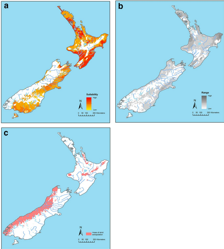
Fig. 2 a Predicted suitability areas for Amblyomma americanum ticks under present-day climatic conditions in New Zealand, as modelled with MaxEnt. White areas are unsuitable and yellow to red areas are increasingly suitable. b Uncertainty associated with the predicted suitability areas for A. americanum ticks under present-day climatic conditions in New Zealand, as modelled with MaxEnt. The uncertainty increases from white to dark grey. c Areas representing strictly extrapolative prediction of suitability for A. americanum ticks under present-day climatic conditions in New Zealand. The red areas are extrapolative and predictions for these areas should be regarded with considerable caution (Owens et al. 2013). (Color figure online)
