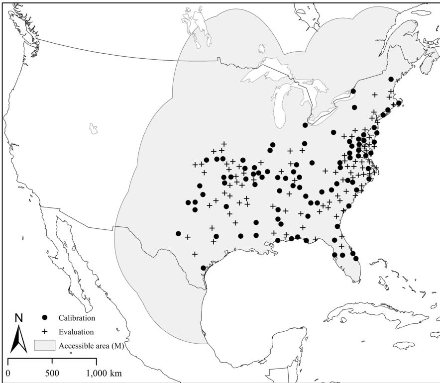
Fig. 1 Points representing 185 georeferenced occurrence records of Amblyomma americanum ticks used in the analysis and a hypothesized area accessible to this species (M) over a period of time. The black dots are the occurrence data points used in the model calibration and the black crosses are the occurrence data points used in the model evaluation
