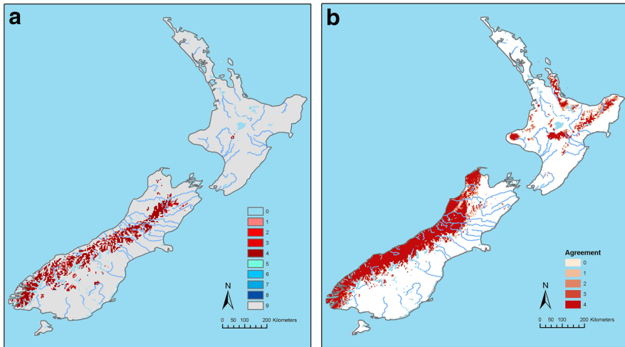
Fig. 3 a The agreement in predicted suitability of areas for Amblyomma americanum ticks between different Global Circulation Models (GCMs) under the Low Emission, Representative Concentration Pathway (RCP) 4.5 Emission Scenario. Where 1 = areas in which one of the four GCMs predicted suitability for A. americanum distribution. 2, 3, 4 = two, three and four GCMs predicted suitability, respectively. 5 = areas in which one of the four GCMs predicted loss of territory for A. americanum compared to the present-day distribution. 6, 7, 8 = two, three, and four GCMs predicted loss of territory, respectively. 9 = no observed change from predicted current A. americanum distribution. b Degree of agreement between Global Circulation Models (GCMs) on extrapolative prediction of suitability areas for A. americanum ticks under the Low Emission, Representative Concentration Pathway (RCP) 4.5 Scenario. Where 1 = Areas in which the prediction based on one of the four GCMs were strictly extrapolative. 2, 3, 4 = degree of agreement in strict extrapolative areas based on two, three and all four models, respectively
