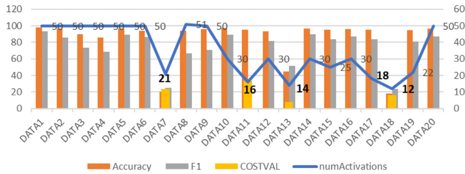
Fig. 5. Detection quality using PSO algorithm.
