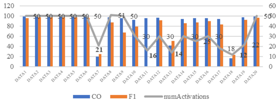
Fig. 6. Detection quality using ASO algorithm.
