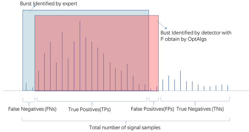
Fig. 3. Confusion matrix for sEMG.
