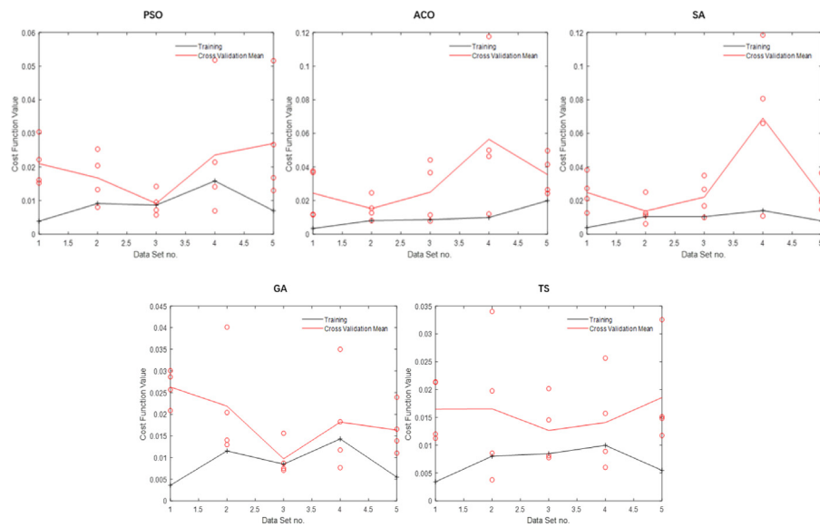
Fig. 7. Obtaining input parameters for detector using cross-validation.
