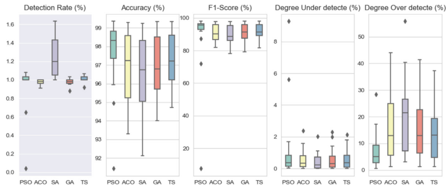
Fig. 9. Comparison of optimization detection results of C2.
