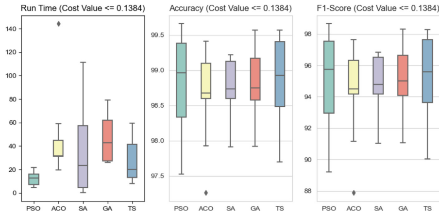
Fig. 10. Distribution comparison of runtime, accuracy, and F1-Score values of the optimization algorithms under the condition of cost value \leq 0.1384 .
