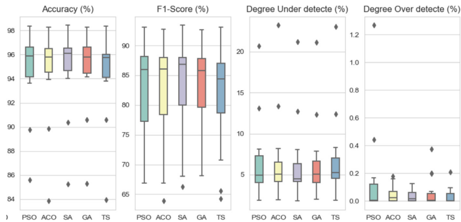
Fig. 8. Comparison of optimization detection results of C1.
