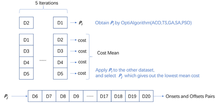
Fig. 2. Cross-validation scheme.
