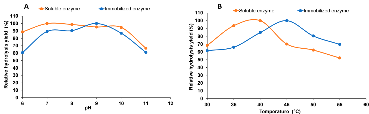
Figure 3. Effect of varying reaction conditions: (A) pH range from pH 6–11 and (B) temperature (30–55 °C) in the hydrolysis of sodium alginate by soluble and immobilized enzyme.
