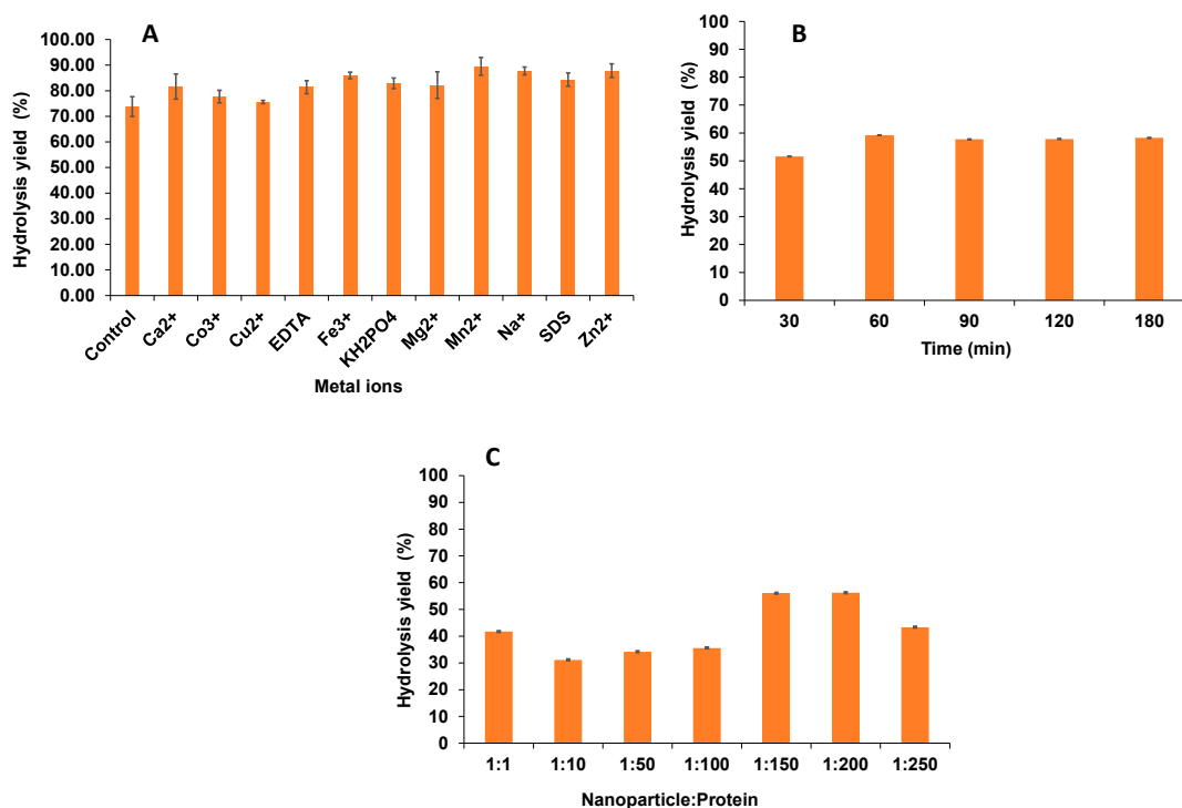
Figure 1. (A) Effect of different metal ions on the enzymatic activity of alginate lyase, (B) Activation of nanoparticles as a function of variable time, (C) Binding efficiency of alginate lyase onto magnetic nanoparticles with varying concentration of protein loaded.
