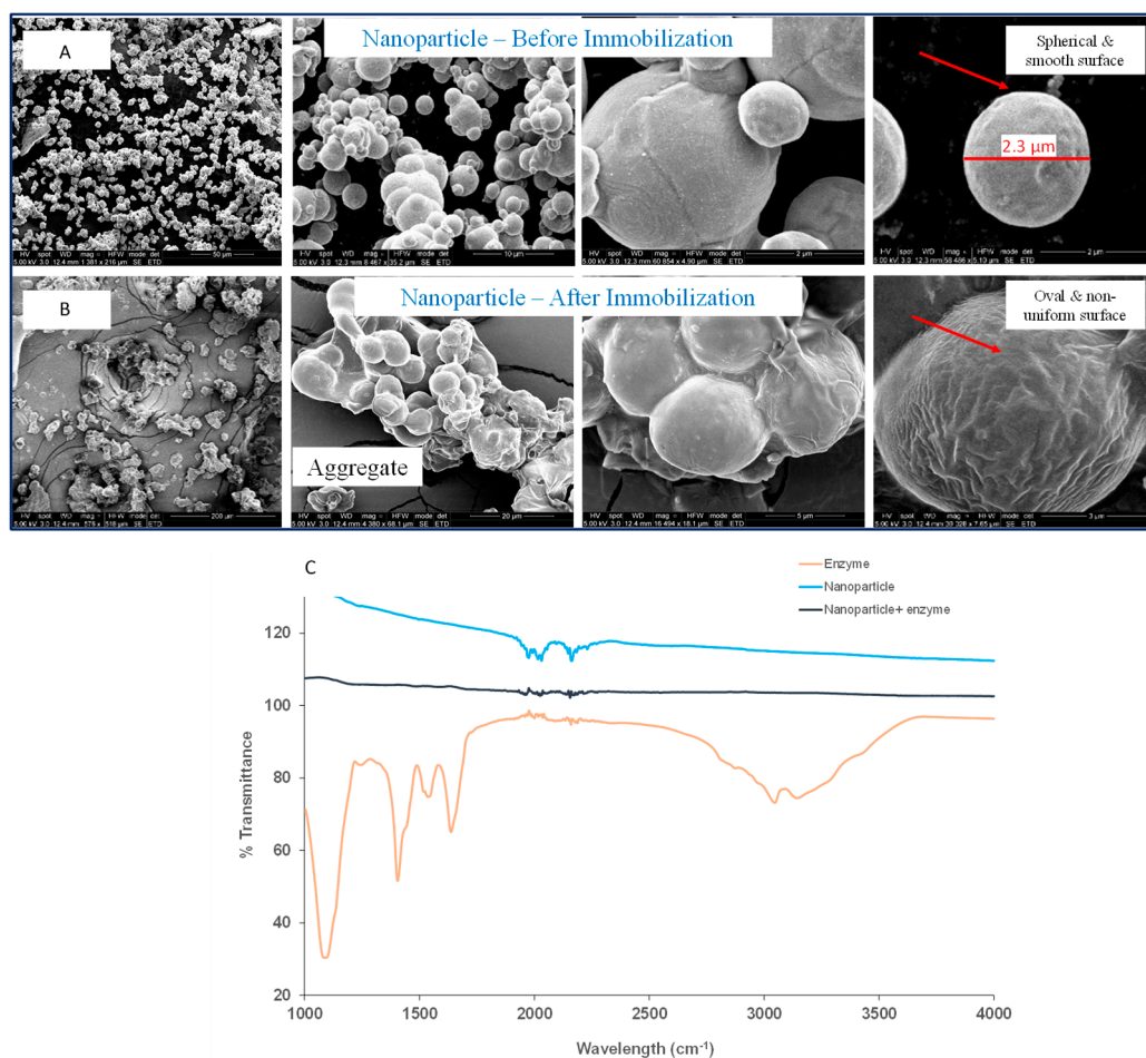
Figure 2. (A) SEM images for nanoparticles and (B) alginate lyase immobilized on nanoparticles at an accelerating voltage of 5 kV and magnification ranges from 500 nm to 300 μm; (C) FTIR spectrum of magnetic nanoparticles, soluble alginate lyase, immobilized alginate lyase.
