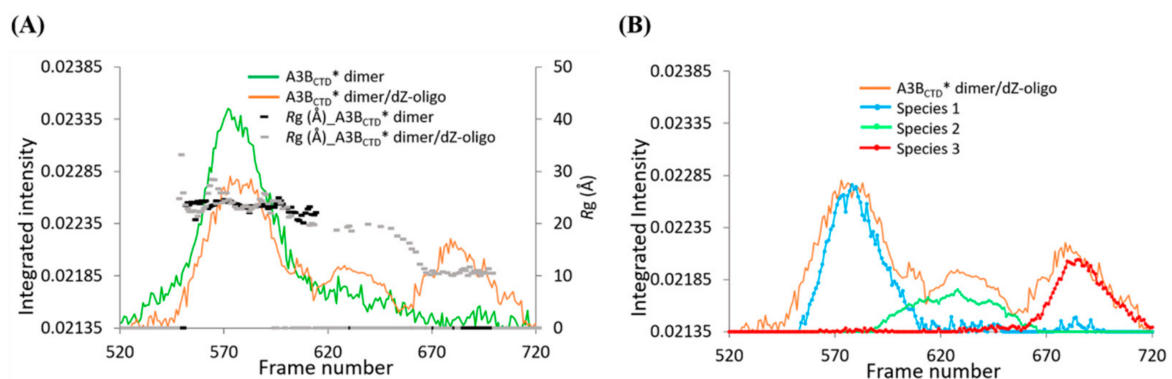
Figure 12. Deconvolution of SAXS data of the A3B CTD * dimer/dZ-oligo. (A) Comparison of the SAXS profiles of the A3B CTD * dimer (green) and A3B CTD * dimer with dZ-oligo at a 1 to 10 ratio (orange) overlaid with Rg trace values. (B) Evolving factor analysis (EFA) analysis using BioXTAS RAW indicating the distinct scattering species 1–3.
