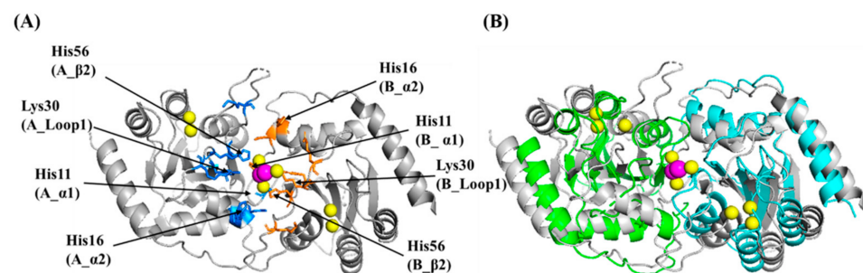
Figure 10. Dimerization interface of A3A-E72A-C171A and A3B CTD *. (A) A3A-E72A-C171A homodimer (PDB 4XXO [49]) (grey) labelled with residues that are important in forming the dimerization interface. A3A molecule A dimerization residues labelled in blue and A3A molecule B dimerization residues labelled in orange. (B) Comparison of the A3A-E72A-C171A homodimer (PDB 4XXO [3,49]) (grey) to our dimer interface model 1 of A3B CTD * (molecule A in green and molecule B in cyan). Zn 2+ ions are represented as yellow spheres and chloride ions are shown as magenta spheres.
