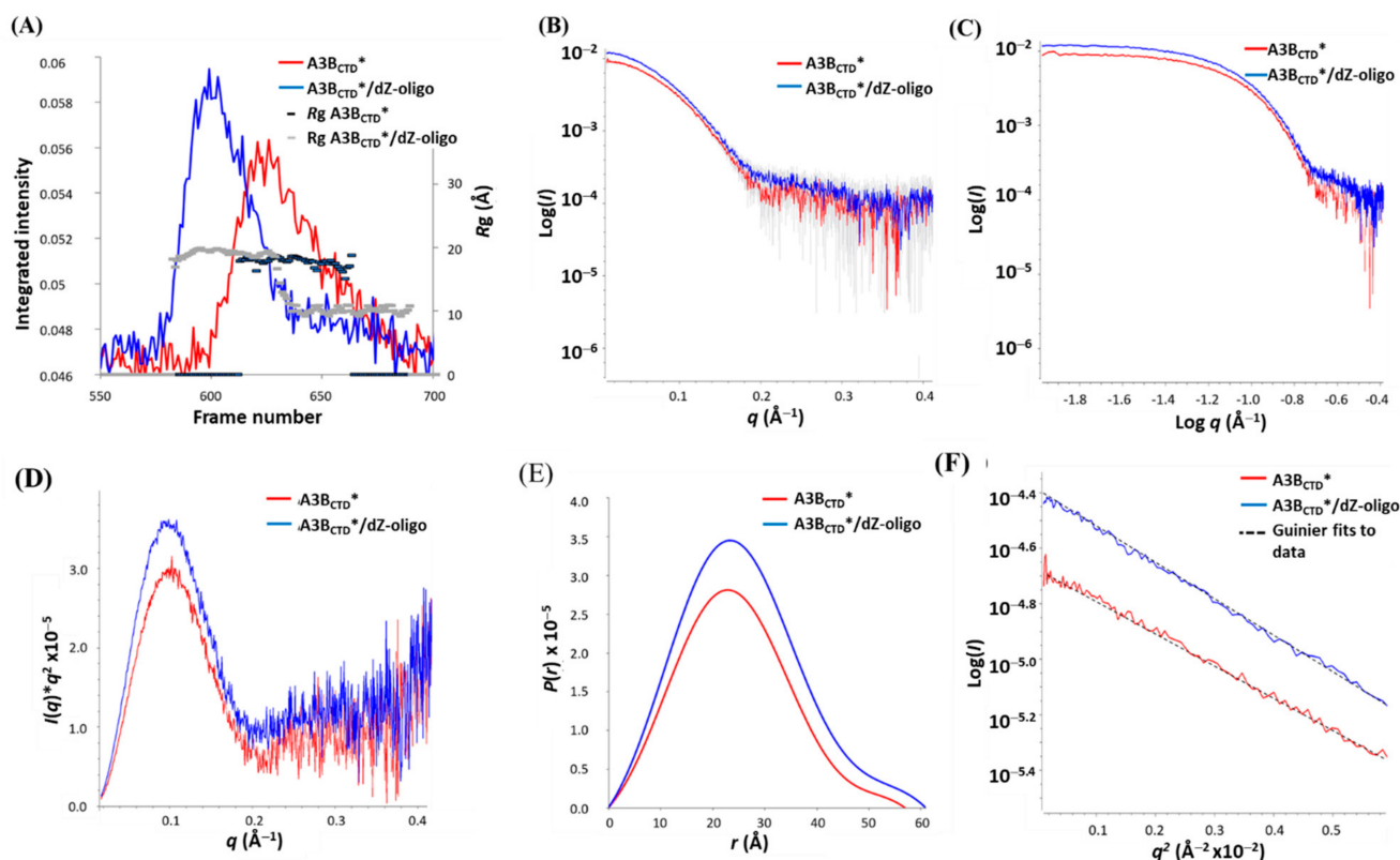
Figure 3. SEC-SAXS analysis of A3B CTD * (red) and A3B CTD */dZ-oligo complex (blue). (A) SAXS profile plots. (B) Scattering curves \log I(q) versus q . (C) Double log plot of scattering. (D) Kratky plot. (E) P(r) distribution plot. (F) Guinier plots. Experiments conducted injecting into SEC-FPLC 5 mg/mL A3B CTD * and A3B CTD */dZ-oligo at a 1 to 2 molar ratio in pH 5.5 buffer (see caption to Figure 2).
