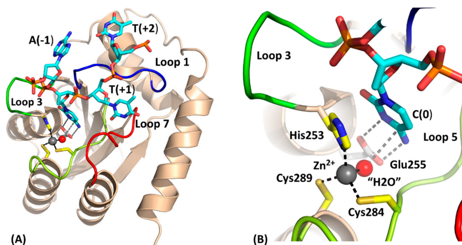
Figure 1. Structure of the catalytically competent C-terminal domain of A3B CTD with ssDNA (PDB code 5TD5). This construct differs from wild-type and is denoted A3B CTD * ( vide supra ). (A) Cartoon representation of the protein with active-site residues shown as colored sticks (red for oxygen, blue for nitrogen, yellow for sulfur and orange for phosphorus). Loops 1 (translated from A3A), 3 (truncated), 5, and 7 are shown respectively in blue, green, limon and red. The general acid-base Glu255 (Ala in structure 5TD5) has been modelled (carbon atoms in light grey) based on the substrate-free active enzyme (PDB code 5CQI). Zn is shown as a grey sphere and the nucleophilic \text{H}_2\text{O}/\text{OH}^- as a red sphere (Note: in crystal structure this is a \text{Cl}^- ). The ssDNA is shown in stick form with carbon atoms distinguished by cyan coloring. Key hydrogen-bonding and incipient nucleophilic attack are shown as dark-grey dashed lines. (B) Magnified view of the active site showing key interactions.
