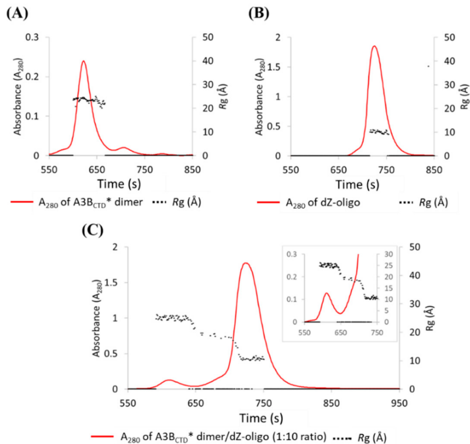
Figure 11. Size-exclusion chromatography (SEC) elution profiles of A3B CTD * dimer and A3B CTD * dimer/dZ-oligo. SEC-FPLC performed using (A) 2.5 mg/mL (~56 \mu M) of A3B CTD * dimer, (B) 1.7 mg/mL (~566 \mu M) of dZ-oligo, and (C) A3B CTD * dimer with dZ-oligo at a 1 to 10 ratio, closeup shown in the insert. Samples were run at 25 ^{\circ} C through a SEC column at a flow rate of 0.2 mL/min in pH 5.5 buffer.
