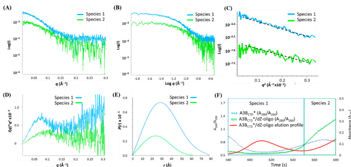
Figure 13. SAXS analysis of the A3B CTD * dimer/dZ-oligo deconvoluted species. (A) 1D-scattering curves of each species. (B) Double log plots. (C) Guinier plots. (D) Kratky plots. (E) P(r) distribution plots. (F) Plots of the absorbance ratio A_{280}/A_{260} to assess presence of ssDNA during elution of the A3B CTD * /dZ-oligo sample. The red line is the elution profile of the A3B CTD * /dZ-oligo sample and the green crosses the A_{280}/A_{260} ratio. The blue crosses are ligand-free A3B CTD * (vide supra). Experiments were conducted using 2.5 mg/mL of A3B CTD * dimer with dZ-oligo at a 1 to 10 ratio in pH 5.5 buffer (see caption to Figure 2).
