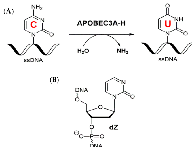
Scheme 1. (A) Deamination of dC in ssDNA by APOBEC3 enzymes. (B) 2'-Deoxyzebarine embedded in ssDNA (as 5'-ATTT-dZ-ATTT) is a low \mu\text{M} inhibitor of APOBEC3.
