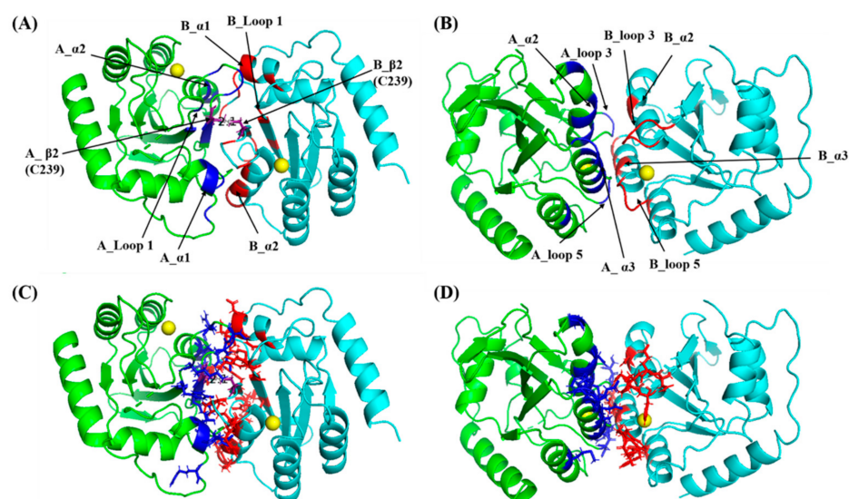
Figure 7. Models of the dimerization interface of A3B CTD *. Predicted interface models between two A3B CTD * molecules using the PRISM 2.0 webserver. A3B CTD * molecule A (green, dimerization interface in blue) and A3B CTD * molecule B (cyan, dimerization interface in red) with Zn 2+ (yellow sphere) in active site. (A,C) Model 1 interface with a calculated \Delta G \sim -38.12 kcal/mol. (B,D) Model 2 interface with a calculated \Delta G \sim -18.6 kcal/mol. Models represented as cartoons in (A,B) have the chains and loops involved in the dimerization interface labelled, whereas in (C,D) residues involved in the dimerization interface are shown in stick format.
