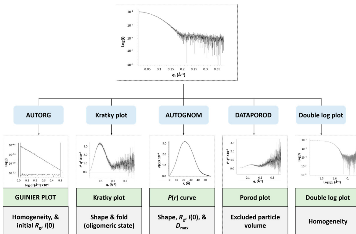
Scheme 3. Schematic of the analysis of SAXS data.
