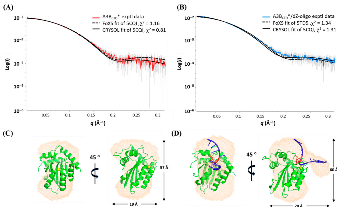
Figure 4. Fitting of experimental (exptl) A3B CTD * SAXS profiles to known A3B CTD crystal structures. (A) Model fit of A3B CTD * to 5CQI crystal structure. (B) Model fit of A3B CTD */dZ-oligo complex (injected into SEC-FPLC in a 1:2 ratio) to 5TD5* crystal structure. (C) Envelope calculated from A3B CTD * SAXS data with 5CQI fitted into the envelope. (D) Envelope calculated from A3B CTD */dZ-oligo SAXS data with 5TD5* fitted into the envelope.
