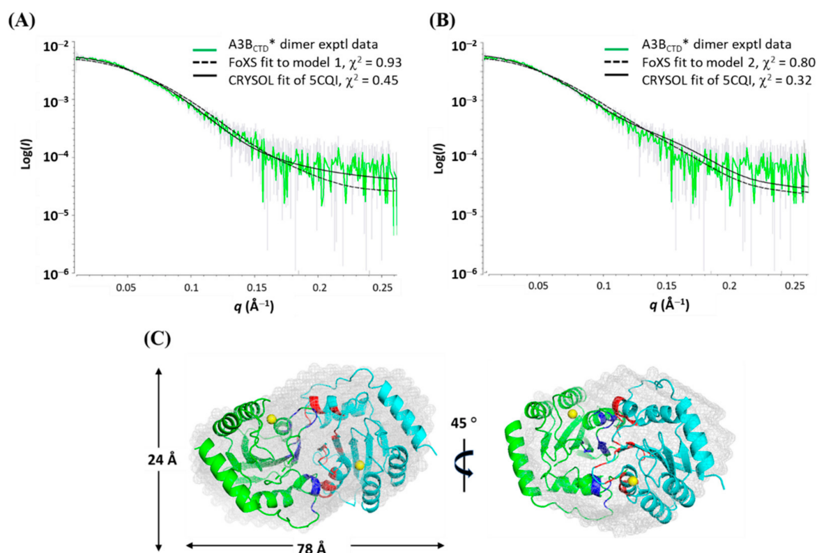
Figure 9. Fitting A3B CTD * dimer scattering data to the simulated atomic interface models. Rigid body modelling of the A3B CTD * dimer to (A) interface model 1 or (B) interface model 2 using FoXS and CRYSOLE. (C) Model 1 interface structure fitted to the A3B CTD * dimer envelope. Averaged envelope model of A3B CTD * dimer derived using P2 symmetry (DAMMIF, DAMAVER and DAMFILT, ATSAS 2.8.3 suite [66]) superimposed with interface model 1.
