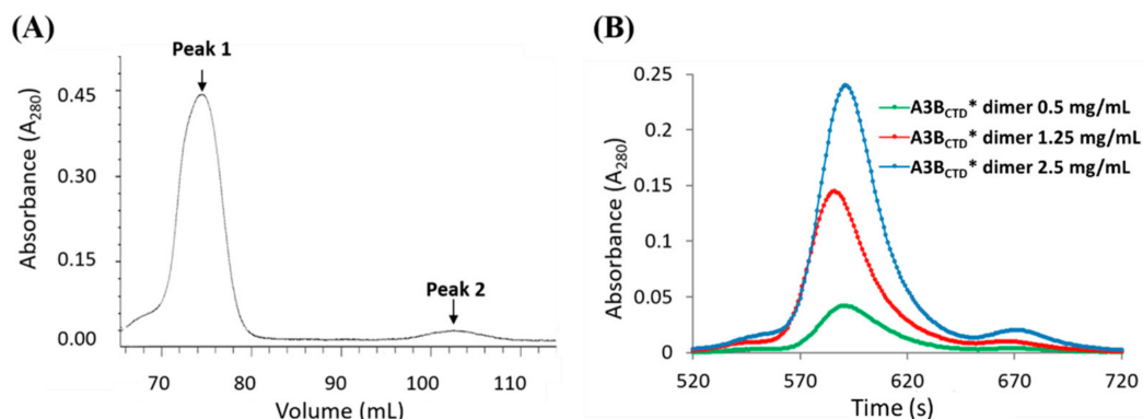
Figure 6. Purification of the A3B CTD * dimer using SEC-FPLC. (A) SEC-FPLC elution profile of 5 mg/mL A3B CTD * dimer. (B) SEC-FPLC elution profiles of the A3B CTD * dimer at varying concentrations 0.5–2.5 mg/mL. SEC-FPLC was conducted at a flow rate of 0.5 mL/min through the SEC column at 25 °C.
