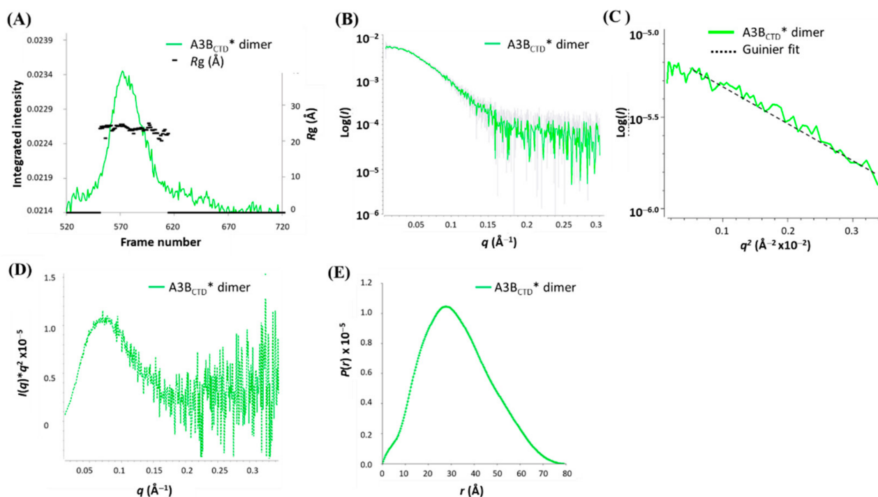
Figure 8. SEC-SAXS analysis of A3B CTD * dimer. (A) SAXS profile plot. (B) scattering curve. (C) Guinier plot. (D) Kratky plot. (E) P(r) distribution plot. Experiments were conducted using 2.5 mg/mL of A3B CTD * dimer in pH 5.5 buffer (see caption to Figure 2).
