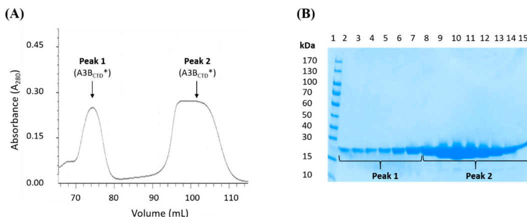
Figure 5. SEC-FPLC purification of the A3B CTD * multimers. (A) SEC-FPLC of A3B CTD * run through a SEC column at a flow rate of 0.5 mL/min at 25 °C, displaying the elution of two forms of A3B CTD *, peak 1 and peak 2. (B) 16% Tricine SDS-PAGE gel (reducing conditions) of the purified A3B CTD * fractions after SEC purification.
