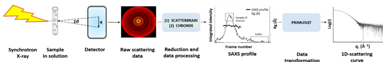
Scheme 2. Schematic representation of a small-angle X-ray scattering (SAXS) experiment and data processing. The scattering vector q is defined as q = 4\pi \lambda^{-1} \sin\theta , 2\theta is the scattering angle, and \lambda is the wavelength of 1.0332 Å for collected data.
