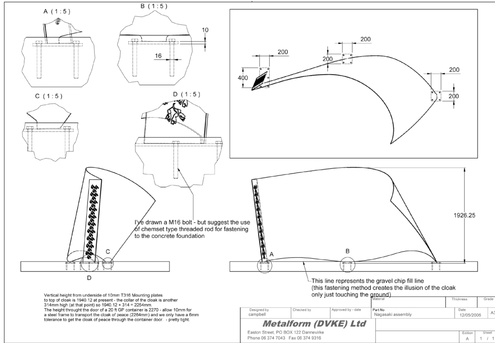
Sculpture installation and layout drawings
