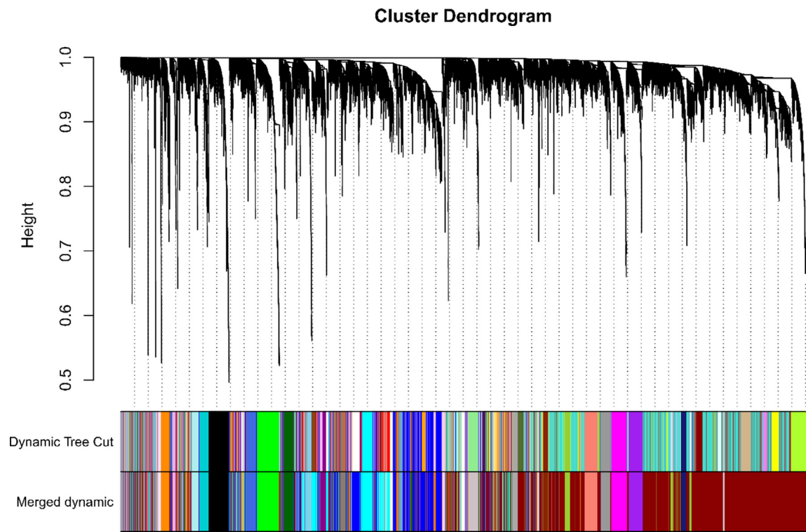
Fig. 3. Module clustering tree diagram. Scale-free networks and topological overlap matrices (TOMs) were constructed. The corresponding TOM phase dissimilarity (diss TOM) was also performed, resulting in the generation of a gene (tree diagram) hierarchical clustering tree based on the function hclust by hierarchical clustering for module detection. In order to avoid generating too many modules, the relevant parameters min Module Size is 30 and deep Split = 2. MEDissThres is set to 0.25, the similarity is 0.75. When the similarity is > 0.75, the modules are merged together to generate new merge the module after that.
