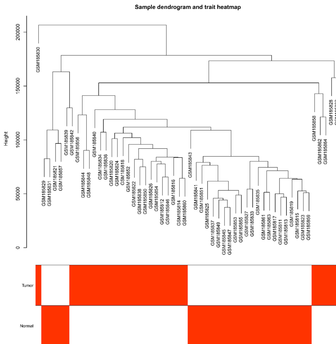
Fig. 2. Sample clustering plot and sample trait heat map. The image is a clustering plot after clustering the samples, and below is a heat map of the samples corresponding to the traits Tumor and Normal, where red indicates the Tumor group. White indicates the Normal group.
