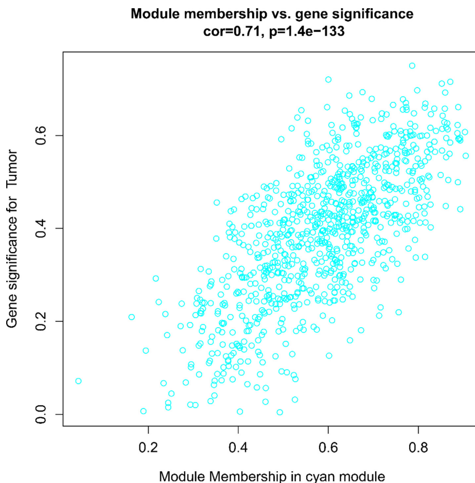
Fig. 5. Scatter plot of correlation analysis of Cyan modules and tumor group. We can see that the correlation coefficient between Cyan module and tumor group reaches 0.71. To find the hub genes associated with the tumor trait, we first calculate the internal connectivity of the gene and the module, which measures the position of the gene within the module, while the module indicates to which module the gene belongs. The higher the correlation between the module MM and the current GS, the more positively the module is correlated with the trait tumor.
