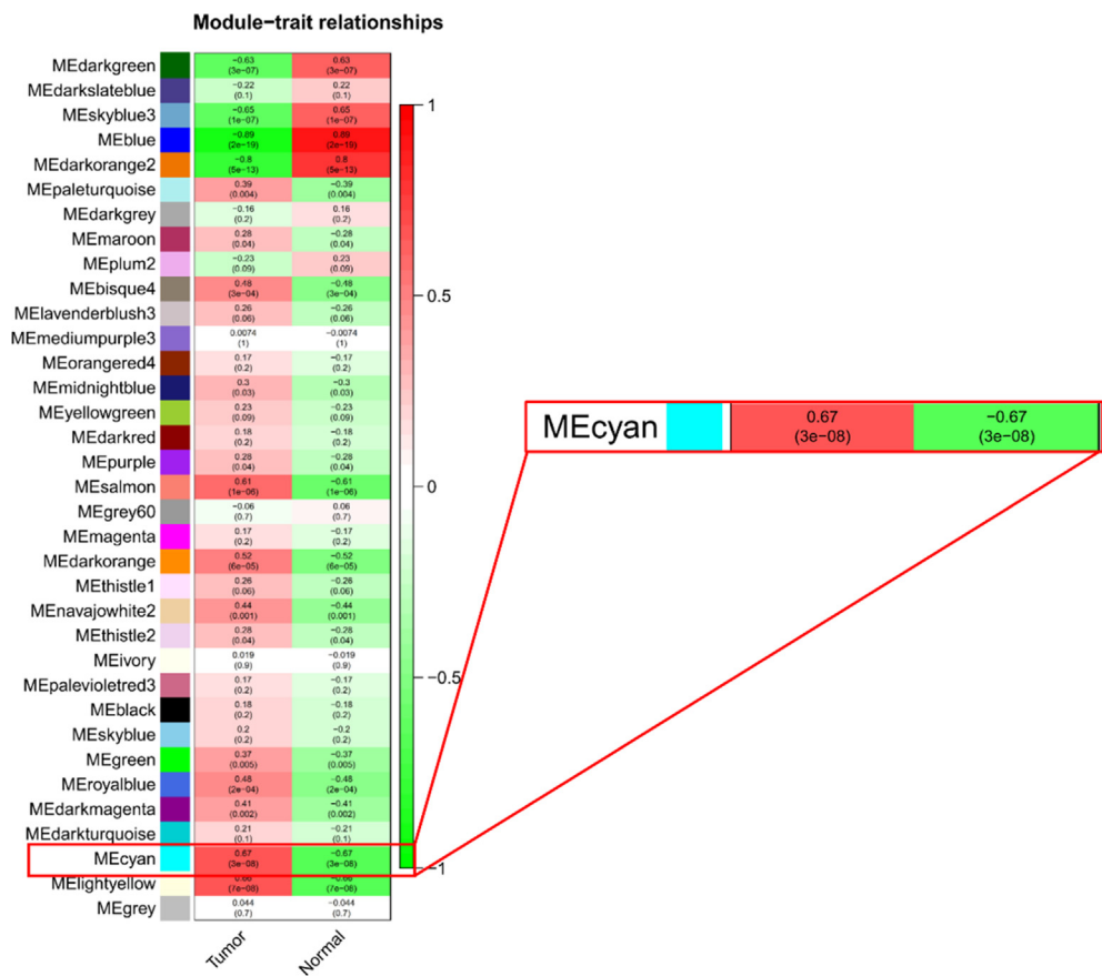
Fig. 4. Module and trait-related heat map. The horizontal coordinates are traits, divided into tumor and normal groups. The vertical coordinates are the clustering obtained for each module. We chose the most correlated (Cor = 0.67, p-value = 3e-08) module cyan for the follow-up study.
