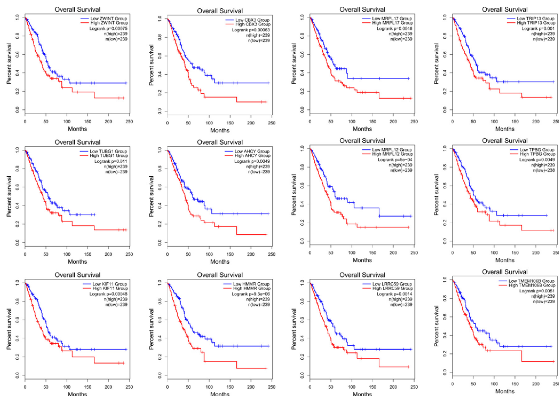
Fig. 8. Survival analysis curves for selected Hub genes. GS correlation in the cyan module was greater than 0.6 for survival analysis, and the clinical sample consisted of 239 low expression groups and 239 high expression groups, method selection overall survival, using median's group cutoff, log rank p < 0.05 .
