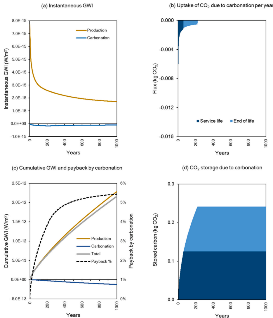
Fig. 3. Baseline DLCA results showing the instantaneous (a) and cumulative (c) GWI over the 1000-year time period and the payback effect of carbonation on it, along with the instantaneous CO 2 uptake (b) and cumulative CO 2 storage (d) by carbonation.
