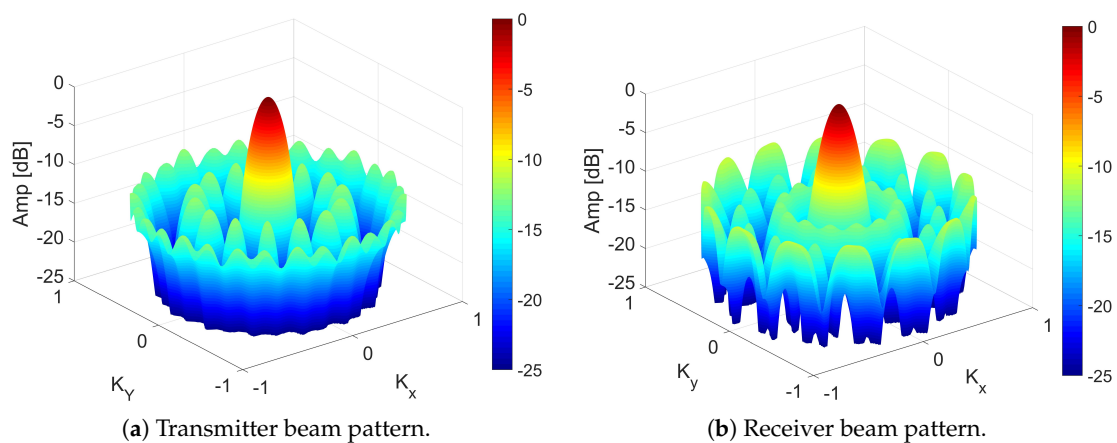
Figure 9. Simulated far-field beam patterns for V1 array at 30 kHz for transmission (a) and reception (b).
