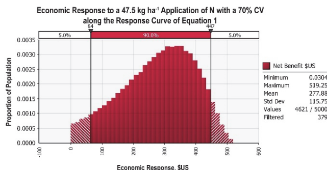
Figure 7. Monte Carlo simulation of net benefit of application of N applied as urea at 47.5 kgNha -1 applied with CV of 70%, and assuming normal distribution application pattern.
