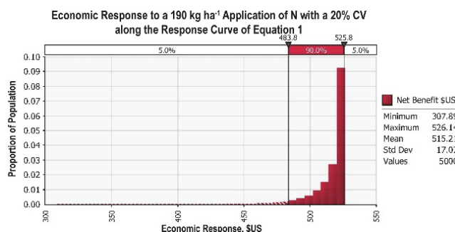
Figure 4. Monte Carlo simulation of net benefit of application of N applied as urea at 190 kgNha -1 applied with CV of 20%, and assuming normal distribution application pattern (fig. 3).
