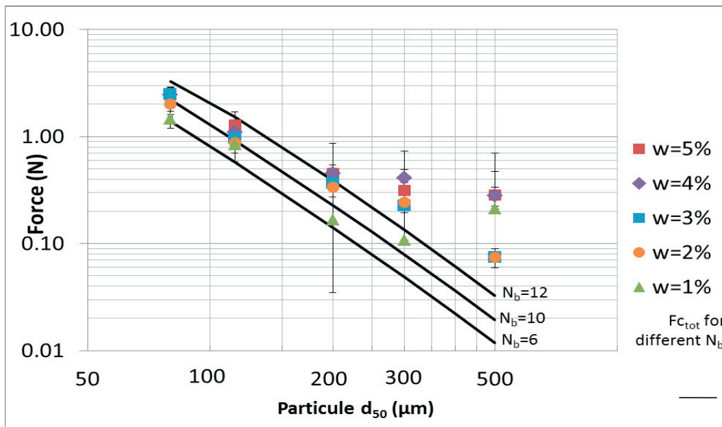
Figure 9: Maximum penetration force measured by the texture analyzer in function of particle size for different water content, compared to the theoretical total capillary force F_{c_{tot}} for different number of bridges ( N_b )
