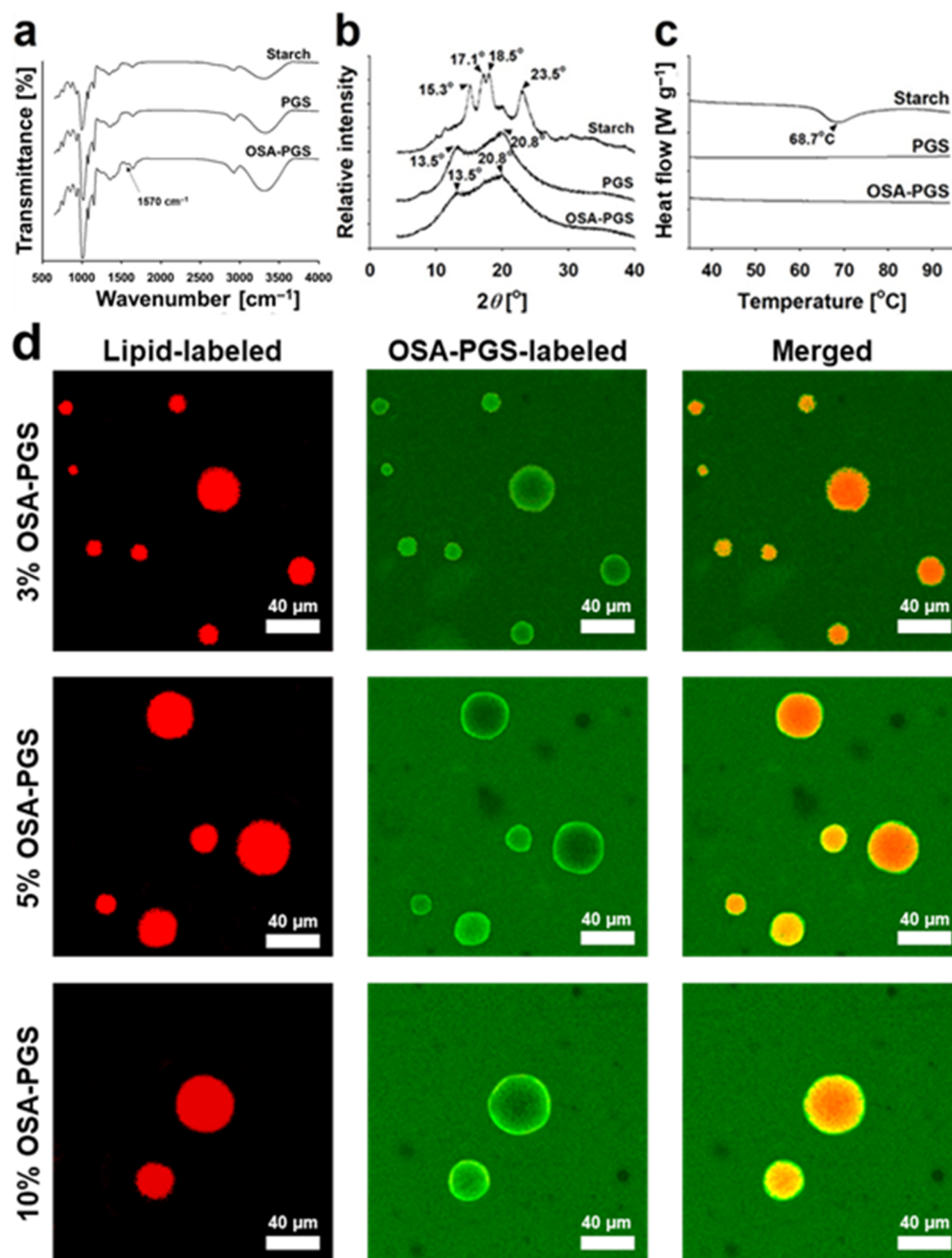
Figure 1. (a) Fourier transform infrared spectra, (b) X-ray diffractograms, and (c) heating calorigrams of maize starch, pregelatinized maize starch (PGS), and octenyl succinic anhydride-modified PGS (OSA-PGS). (d) Confocal laser scanning micrographs of emulsions stabilized by 3, 5, or 10% w/v OSA-PGS and oil volume fraction = 0.05 (Nile red, lipid-labeled; Concanavalin A conjugated with fluorescein isothiocyanate, OSA-PGS labeled).
