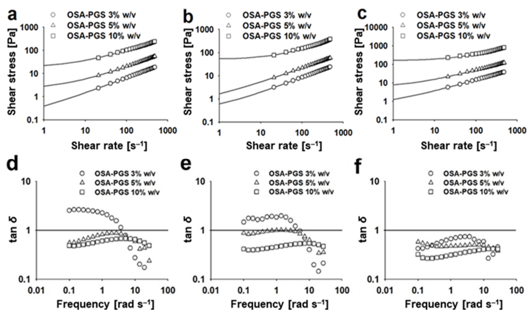
Figure 2. Flow behavior plots (shear stress vs. shear rate) of the emulsions stabilized by pre-gelatinized maize starch modified with octenyl succinic anhydride (OSA-PGS). Oil volume fraction: (a) 0.05, (b) 0.10, and (c) 0.20. Lines indicate the fitted curves based on the Herschel-Bulkley model ( \tau = \tau_0 + K\dot{\gamma}^n ; \tau , shear stress; \dot{\gamma} , shear rate; \tau_0 , yield stress; K , consistency index; n , flow index). Loss tangent angles ( \tan \delta = G''/G' ; G'' , loss modulus; G' , storage modulus) of the emulsions stabilized by OSA-PGS. Oil volume fraction: (d) 0.05, (e) 0.10, and (f) 0.20. Data were obtained by oscillation frequency sweep test. Lines indicate \tan \delta = 1 .
