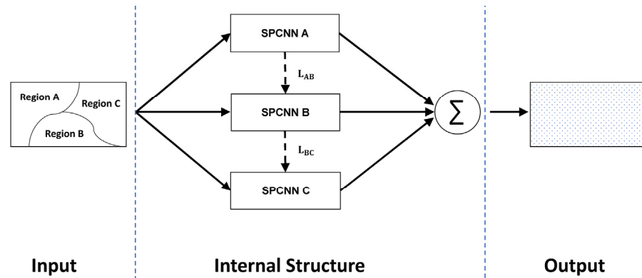
Figure 4. Structure of group-linked HSPCNN.
