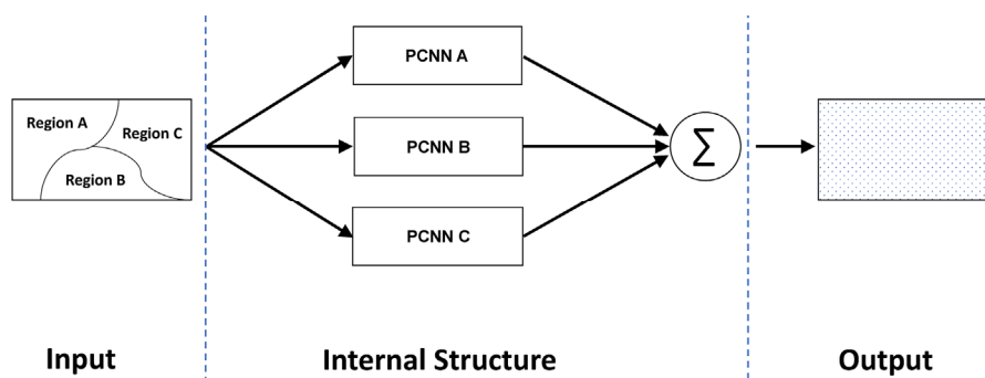
Figure 3. Structure of group-isolated HPCNN.
