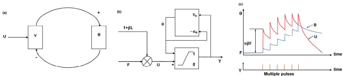
Figure 2. Schematic of the pulse-coupled neural network. (a) Connection between the internal activity U_{ij} , timing pulse sequence Y , and dynamic threshold \theta_{ij} . (b) Schematic of the PCNN. (c) Activity of the internal activity U_{ij} and dynamic threshold \theta_{ij} under stimulation of multiple pulses.
